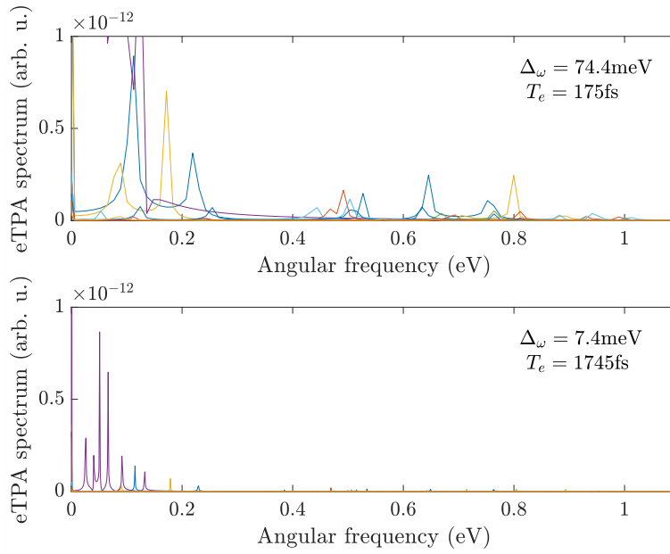
Figure 6: eTPA spectra for ten random sets of two intermediate states each for two different choices of \Delta_\omega ( T_e ) at constant \Delta_L = 45 \text{ nm} and pump wavelength \lambda_p = 405 \text{ nm} . We observe that a small bandwidth leads to strong attenuation of peaks at frequencies far from the resonance (bottom), yet a large bandwidth results in poor resolution in \omega (top).
