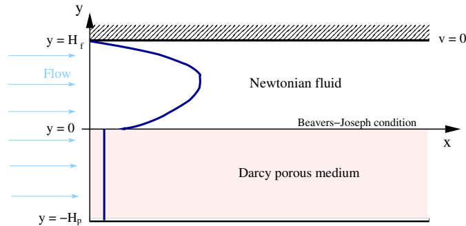
FIGURE 2. Two-layer configuration for Poiseuille flow overlying a porous medium (Darcy): velocity is significantly discontinuous at interface
