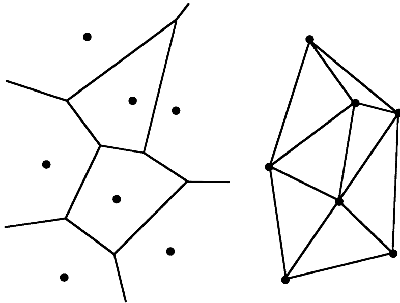
A Voronoi diagram and the corresponding Delaunay triangulation.
