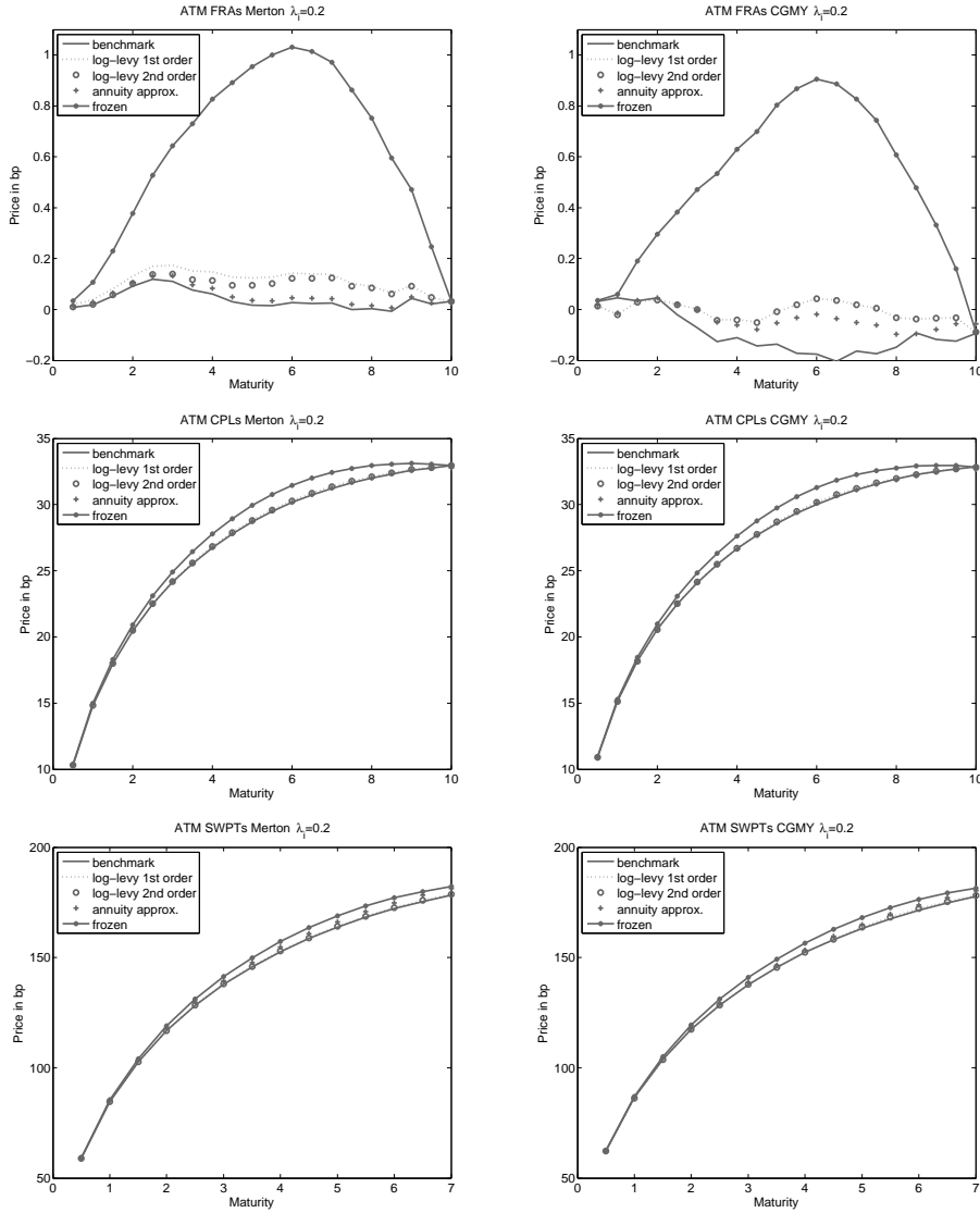
FIGURE 5.3. Prices for the Merton and CGMY models.
