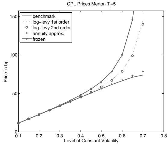
FIGURE 6.2. Caplet prices as a function of volatility ( N = 10 ).
