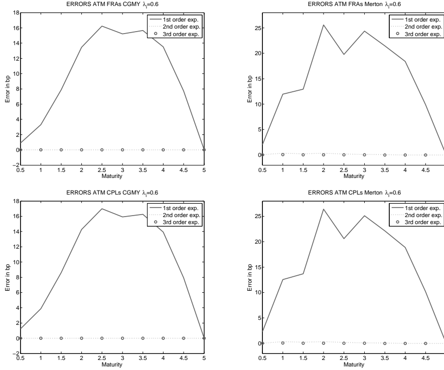
FIGURE 5.2. Drift expansion: high volatility scenario.
