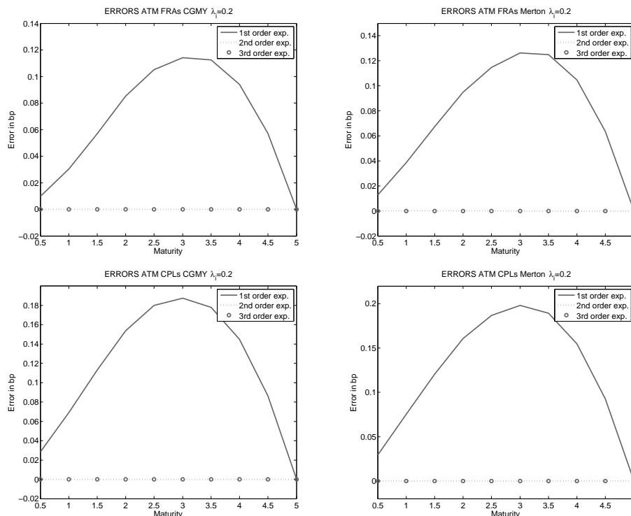
FIGURE 5.1. Drift expansion: low volatility scenario.
