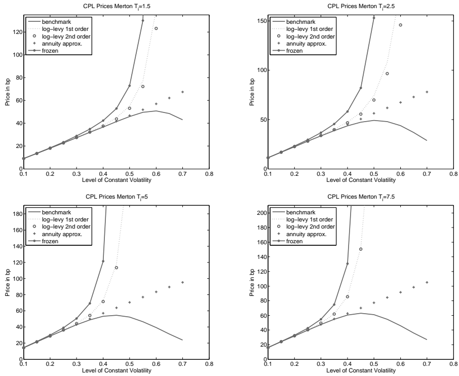
FIGURE 6.1. Caplet prices as a function of volatility ( N = 20 ).
