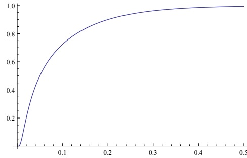
Figure 3: Normalized distribution function \tilde{u}(\tilde{t}, 0.5) for \gamma = -1/4
