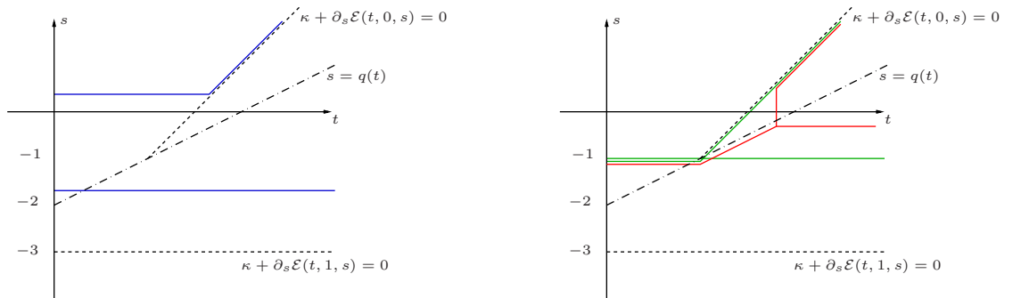
Figure 4.2: Graph of local energetic solutions. More precisely, in the figure on the left, the blue lines correspond to local energetic solutions with initial condition s_0 > -1 and s_0 < -1 . In the figure on the right, we depicted some solutions starting from s_0 = -1 .
