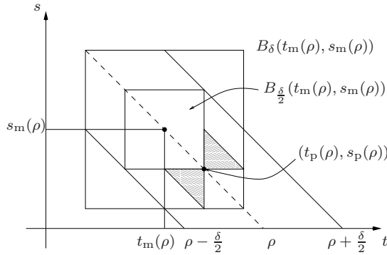
Figure 5.1: If (t_p(\rho), s_p(\rho)) belongs to the boundary of the square B_{\frac{\delta}{2}}(t_m(\rho), s_m(\rho)) , then for every \tilde{\rho} \in [\rho - \frac{\delta}{2}, \rho + \frac{\delta}{2}] the pair (t_p(\tilde{\rho}), s_p(\tilde{\rho})) belongs to the two shaded triangles, both contained in the largest square B_\delta(t_m(\rho), s_m(\rho)) .
