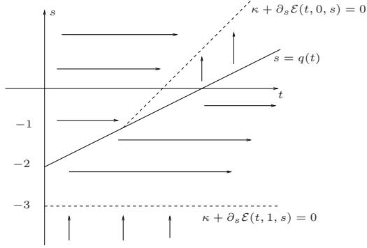
Figure 4.1: The behavior of a local energetic solution: sticking above the line \kappa + \partial_s \mathcal{E}(t, 0, s) = 0 , and jumping in the region between \kappa + \partial_s \mathcal{E}(t, 0, s) = 0 and s = q(t) . Again sticking in the region between s = q(t) and \kappa + \partial_s \mathcal{E}(t, 1, s) = 0 , and jumping below the line \kappa + \partial_s \mathcal{E}(t, 1, s) = 0 .
