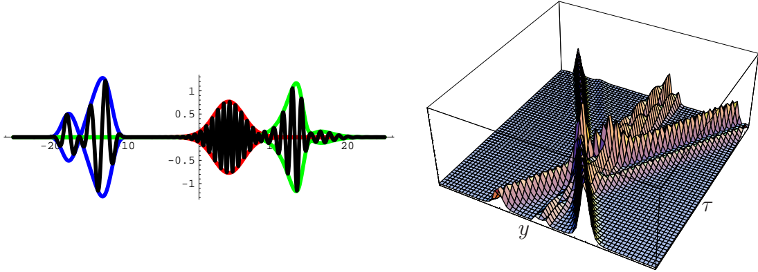
Figure 3.1: Left: typical initial condition. Right: energy distribution in space-time.
