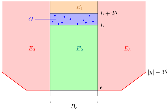
FIG. 3. Illustration of the regions G, E^1, E^2 and E^3 , as in (2.9).
