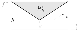
FIG. 1. Illustration of \mathcal{H}_h^s .
