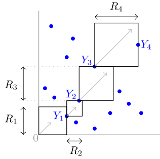
FIG. 5. Illustration of choosing R_1, R_2, R_3, R_4 and Y_1, Y_2, Y_3, Y_4 .
