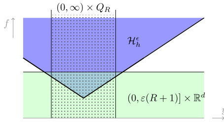
FIG. 2. Illustration (0, \infty) \times Q_R \subset \mathcal{H}_h^\varepsilon \cup (0, \varepsilon(R+1)] \times \mathbb{R}^d .
