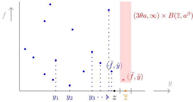
FIG. 4. Visualisation of z, \bar{z} and (\tilde{f}, \tilde{y}) (for d = 1 ).
