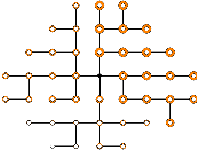
Figure 7. Network topology of the large sized network for the example of truncated Gaussian exit demand. Illustration of the solution of the capacity maximization at exit points for the probability level of p = 0.80 . The entry and exit points are displayed as before. The picture shows the allocated free capacities obtained at the particular exit nodes of the network. Quantities are highlighted by colored circles of different size.
