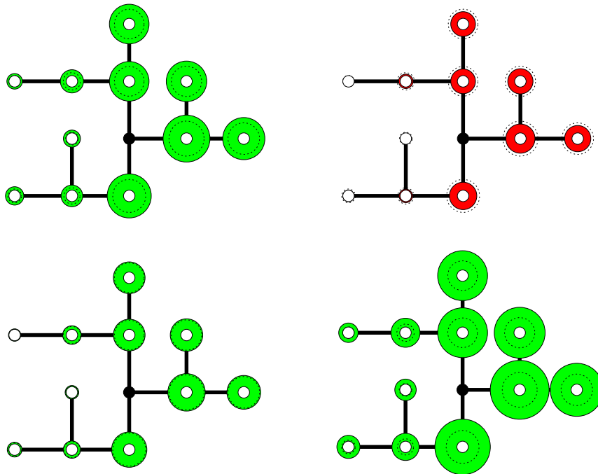
Figure 6. Four simulated exit demand realizations according to the chosen multivariate Gaussian distribution and the respective available free capacity compared to the allocated capacity provided by the numerical solution for the medium network for the probability level p = 0.80 . Feasible and infeasible situations are displayed in green and red, respectively.
