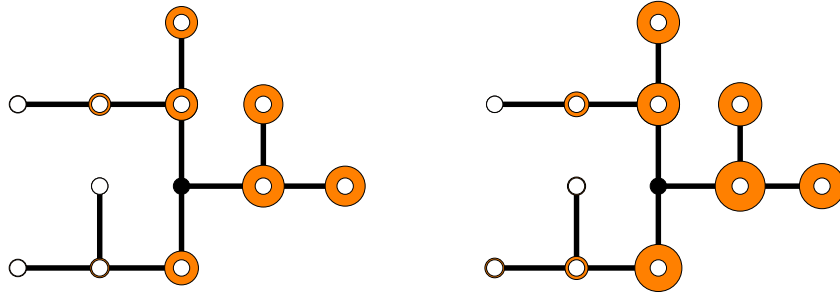
Figure 5. Network topology of a medium sized gas net for the example of Gaussian exit demand. Illustration of the solution of the capacity maximization at exit points for different probability levels p = 0.90 (left) and p = 0.80 . The entry and exit points are displayed in black (entry) and white (exit), respectively. A decreasing probability level allows for a higher allocation of capacities in certain regions of the network highlighted by colored circles of different size.
