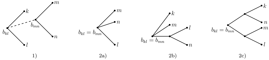
Figure 2. Pictograms for the case study in order to prove Theorem 4.6.
