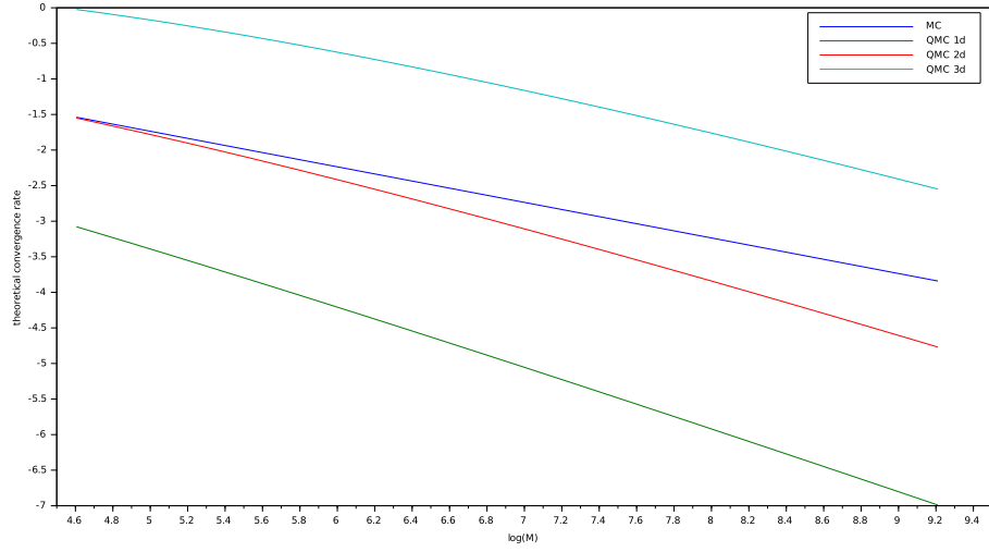
Figure 3.3: Comparison of the theoretical convergence rate for the Monte Carlo and Quasi Monte Carlo methods, up to dimension three. We can observe that, for a relatively small number of simulations (up to 10^4 ), MC converges faster (in theory) than QMC in dimension 3.
