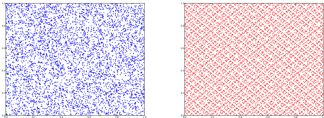
Figure 3.1: Pseudo random samples in [0,1]^2 (left picture) versus quasi random ones (right picture)
