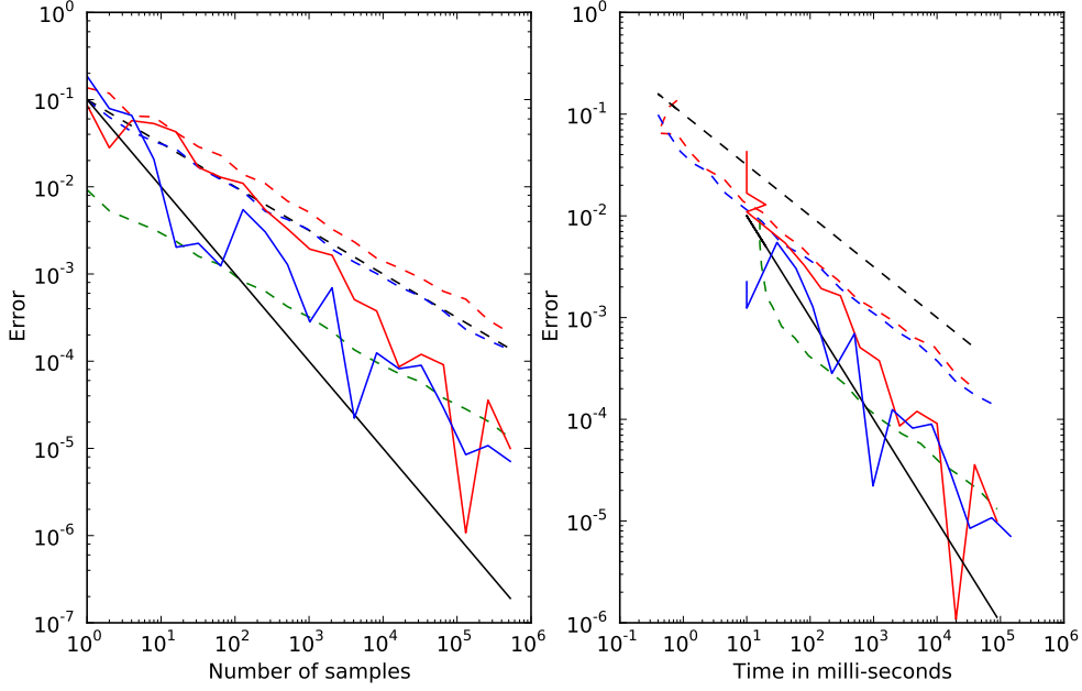
Figure 3.5: The Asian option from Exercise ?? using Monte Carlo and Quasi Monte Carlo simulation (Solid lines: QMC simulation, dashed lines: MC simulation; Red: normal simulation, blue: antithetic variates, green: control variates, black: references line proportional to 1/M ).
