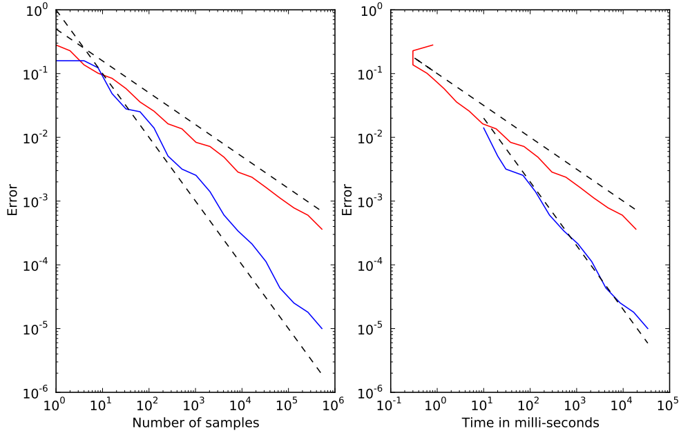
Figure 3.4: A call option in the Black-Scholes model using Monte Carlo and Quasi Monte Carlo simulation. Red: MC simulation, blue: QMC simulation, black: Reference lines proportional to 1/M and 1/\sqrt{M} .
