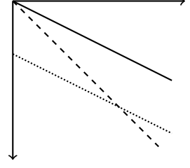
Figure 2.4: Improved convergence rate vs. improved constant.
