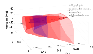
Fig. 2: Bifurcation diagram for the reduced model
