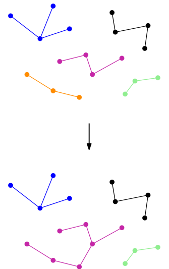
Fig. 5: Transition of the cluster configuration in the inhomogeneous random graph
