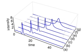
Fig. 3: Soliton solutions of the NDDE model (a)
