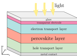
Fig. 3: Perovskite solar cell
