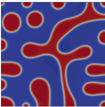
Fig. 2: Late-stage VPS: Volume-preserving curvature flow induced by square-root of the minus Laplace–Beltrami
