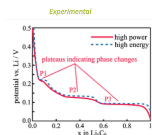
Figure 2: Graphite, in M. Ender et al., Journal of Power Sources 269 (2014) 912-919
