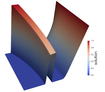
Fig. 3: Solution of the problem that models the transport of a concentration through a domain; the inlet ( x = 0 ) is on top and the outlet ( x = 1 ) at the bottom
