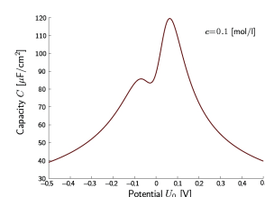
Fig. 1: Capacity as a function of the applied voltage. Each point relies on the complete distribution of the constituents on the interface and within the electrolytic layer
