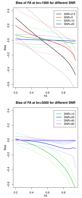
Fig. 3: Bias of FA in nonlinear regression diffusion tensor models for varying SNR. Top: b -value 1000s/mm^2 , bottom: b -value 3000s/mm^2 . Dotted lines are 0.1 and 0.9 quantiles.
