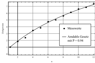
Fig. 2: Amdahl's law
