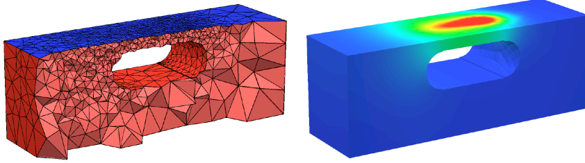
Figure 10: An adaptive tetrahedral mesh (left) and the calculated numerical solution (right) of a heat conduction problem.
