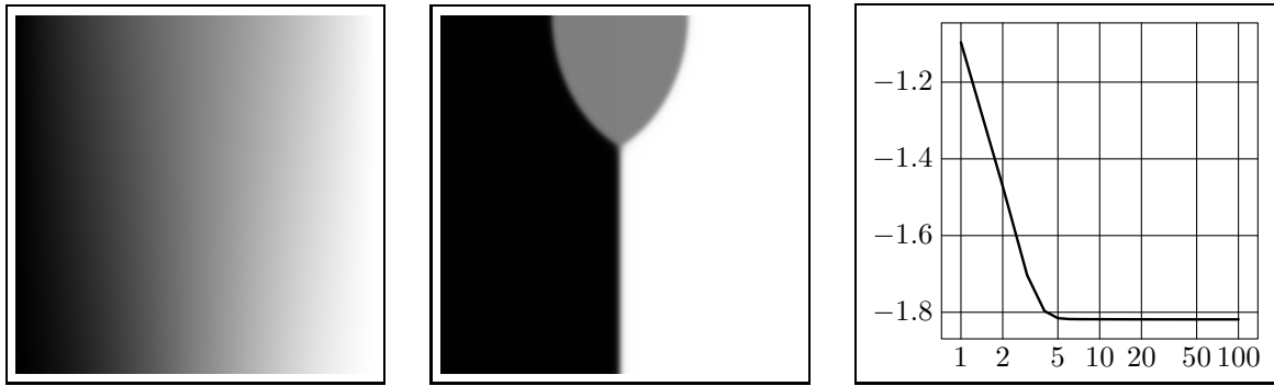
FIGURE 2. Phase separation: (a) mirror-symmetric initial value; (b) final state (phases separated by two arcs and a straight line); (c) decay to the global minimum of the free energy functional F after 100 iteration steps.
