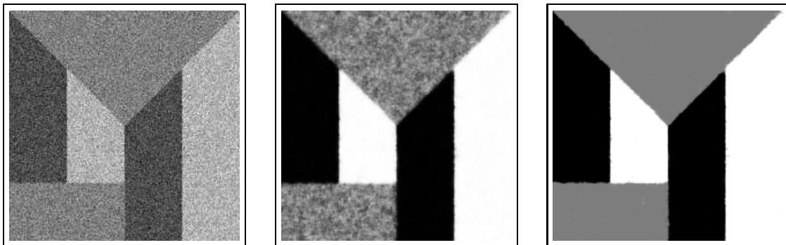
FIGURE 4. Image reconstruction: (a) initial value (noisy image); (b) final state of the two-component black and white reconstruction (gray region still noisy); (c) final state of the three-component reconstruction.
