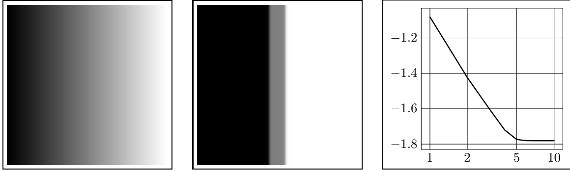
FIGURE 1. Phase separation: (a) initial value (constant in vertical direction); (b) final state (stripe pattern); (c) decay to the corresponding local minimum of the free energy functional F after 10 iteration steps.
