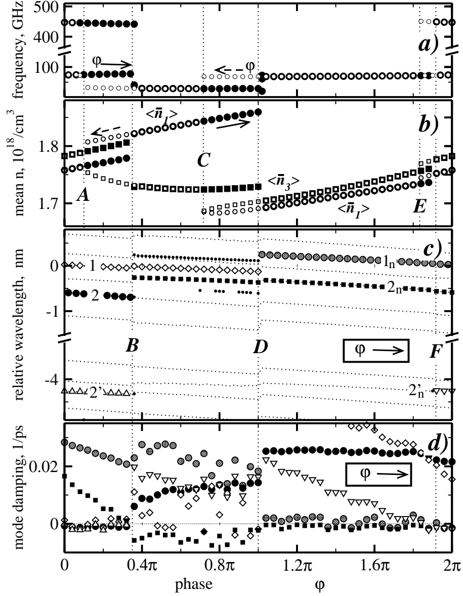
Figure 10: Phase tuning characteristics of a PhaseCOMB laser. Panels a and b : simulation calculations for decreasing (empty symbols) and increasing (full symbols) phase \phi . Panel a : frequencies of the dominant peaks in the rf power spectrum (left facet); only side peaks suppressed by \leq 10\text{dB} are considered. Panel b : spatio-temporal averages of carrier densities in DFB 1 (bullets) and DFB 2 (squares). Panel c : wavelengths of all modes in the given spectral range (dotted lines). Big symbols indicate positions of dominant peaks (differing by \leq 10\text{dB} ). The medium symbols in interval [B, D] represent four-wave mixing side peaks, which are suppressed by \leq 40\text{dB} here. Panel d : damping \Im m\Omega of important modes. The same symbols as in panel c are used but side modes are also shown.
