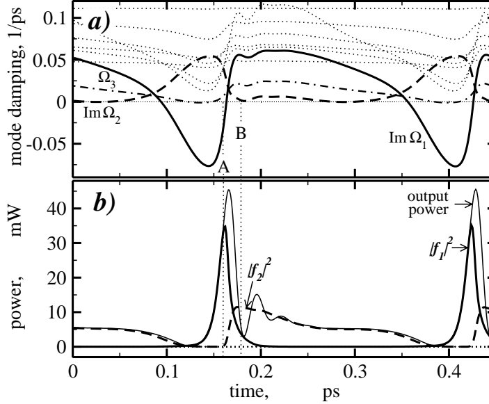
Figure 6: Mode analysis of the pulsating state drawn in Fig.3a. Panel a : evolution of modal decay rates. Solid, dashed and dash-dotted: modes which sometimes reach zero or negative damping. Thin dotted: modes with always positive damping. Labeling as in Fig. 5. Panel b : evolution of the output field power (thin solid) and modal amplitudes. Solid and dashed bold lines: the two most prominent modal contributions.
