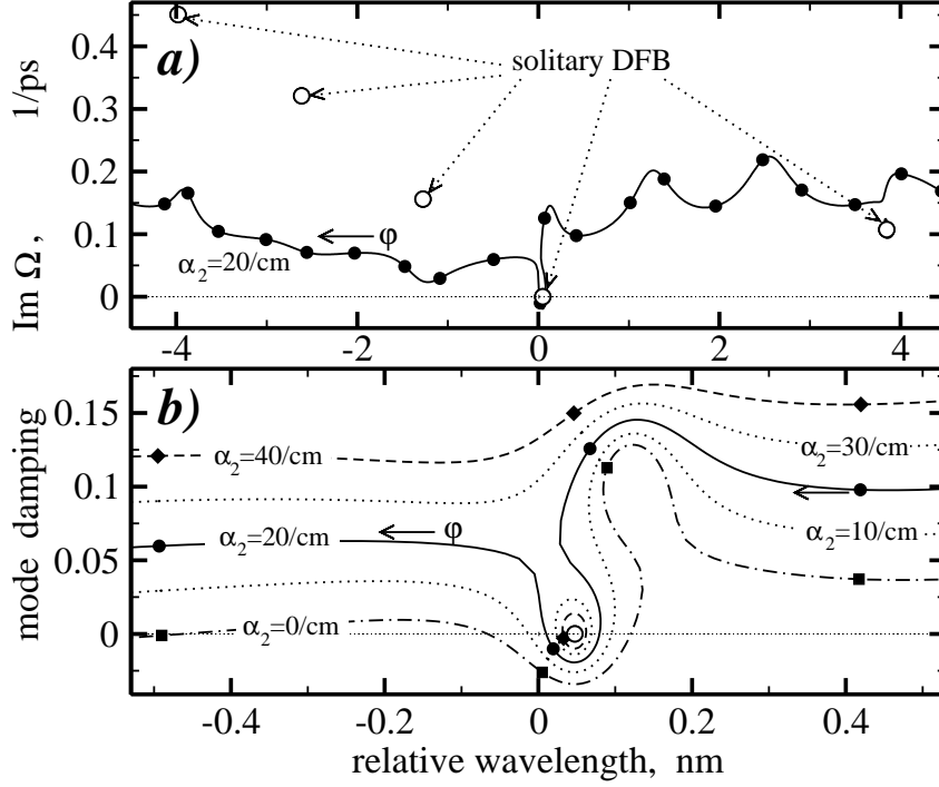
Figure 4: Spectrum of optical modes. Abscissa: relative wavelength (-\Re\Omega \cdot \lambda_0^2/2\pi c_0) . Panel a : overview. Panel b : the modes close to resonance. Lines: location of eigenvalues for all possible \varphi and different optical losses \alpha_2 in the passive section. Arrows: direction of increasing \varphi . Full symbols: modes at \varphi = 0 . Empty bullets: modes of the solitary DFB laser.
