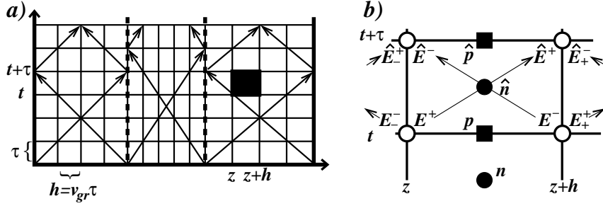
Figure 11: Discretization of the spatial-temporal domain. Panel a : full domain overview. Panel b : positions (solid symbols) where grid functions are defined and their notations in the neighbourhood of one cell (black box in panel a of this figure) of the mesh.
