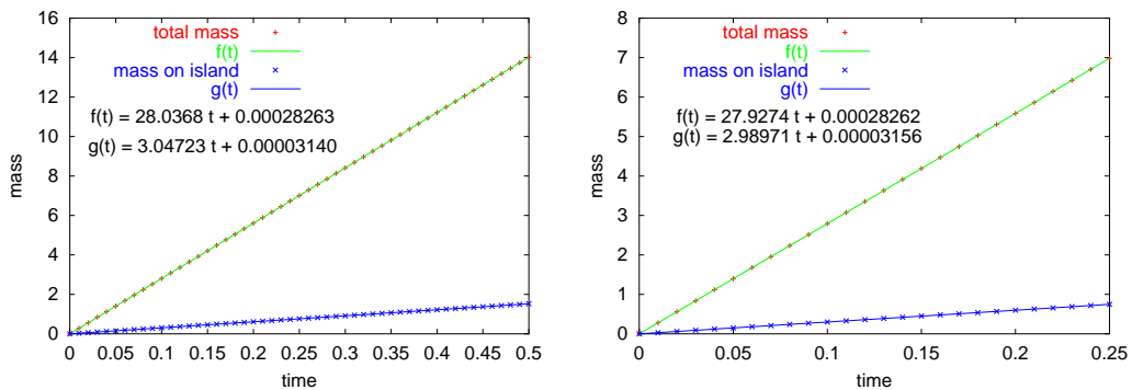
Figure 11: Mass increase: circular island (left) and perturbed circular island (right).
