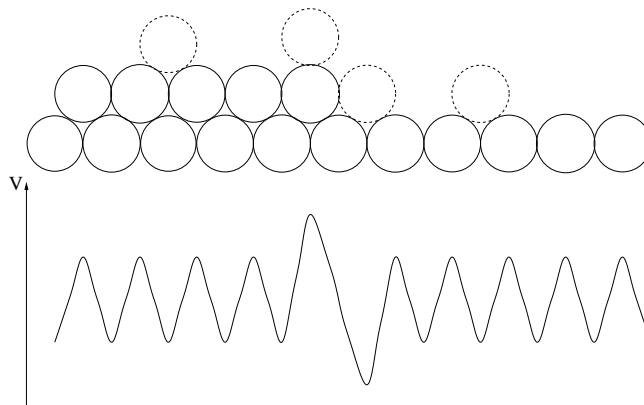
Figure 1: The Ehrlich-Schwoebel barrier.
