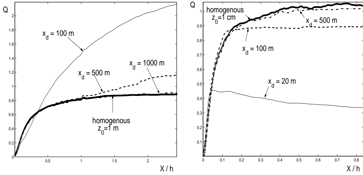
Figure 15: The same as in Figure 13, but for the cumulative footprint function of flux Q .
