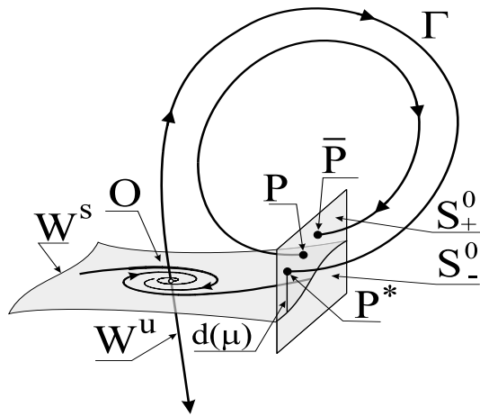
Figure 4: The Poincaré map T : S^0_+ \rightarrow S^0 is defined near S^0 \cap W^s . The image T(W^s \cap S^0) = P^* is defined by continuity. The point P^* = \Gamma \cap S^0 lies on the distance |d(\mu)| from S^0 \cap W^s .
