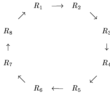
Figure: Catalytic reaction cycle ( M = 8 )
