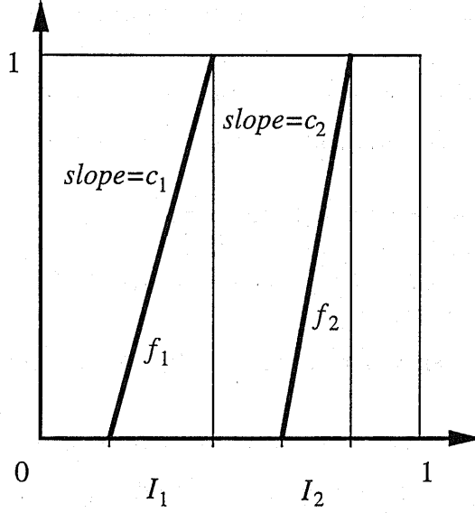
FIGURE 5. A one-dimensional linear Markov map of the unit interval.
