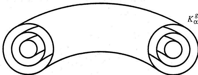
FIGURE 1. A typical multifractal decomposition for a smooth function g .
