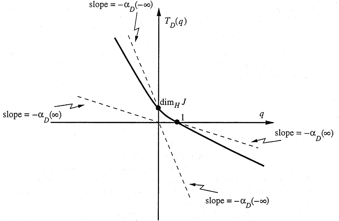
FIGURE 3. A typical graph of the function T_D(q) .
