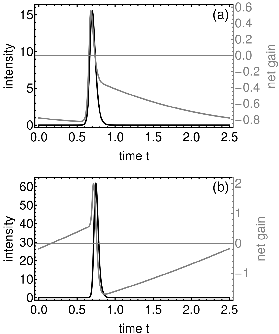
Figure 4: Pulse amplitude a^2 (black line) and net gain (gray line) obtained with the generalized Haus model (26) as functions of the fast time t . (a) – g_0 = 1.0 ; (b) – g_0 = 3.0 . Other parameters are the same as in Fig. 1.
