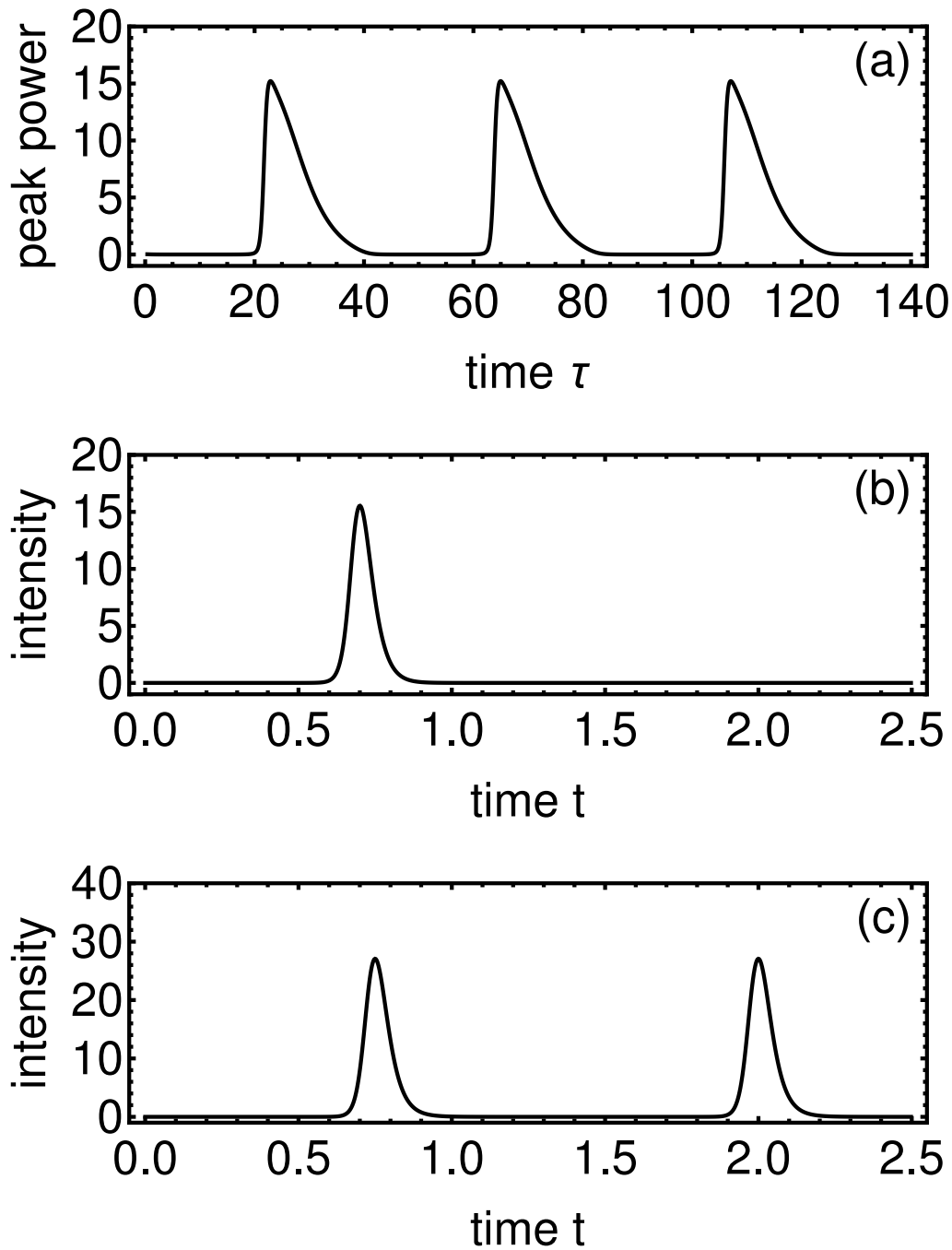
Figure 2: Time traces obtained by numerical integration of the generalized Haus model, Eqs. (26). (a) – g = 0.3 , pulse peak power of the Q-switched mode-locking regime as function of slow time \tau . (b) – g_0 = 1.0 , intensity a^2 of the fundamental mode-locked regime as function of the fast time t . (c) – g = 3.0 , intensity a^2 of the harmonic mode-locking regime with two pulses per cavity round trip as a function of the fast time t . Other parameters are the same as in Fig. 1
