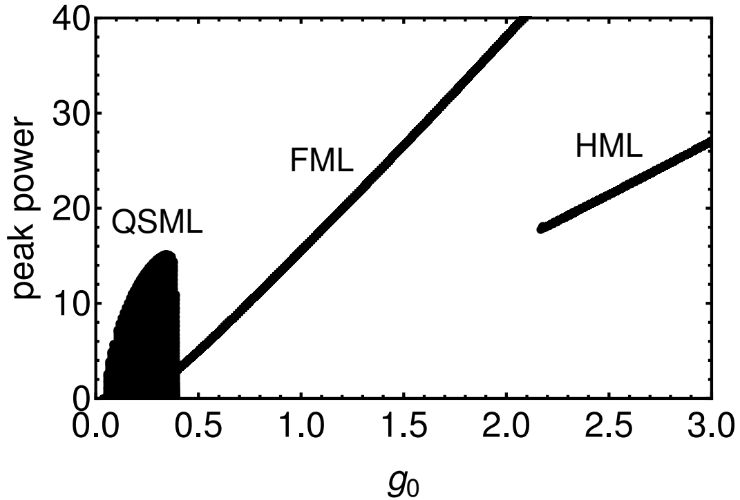
Figure 1: Pulse peak power a^2 as a function of the pump parameter g_0 obtained using the generalized Haus model, Eqs. (26). QSML, FML, and HML denote Q-switched, fundamental, and harmonic (with two pulses per cavity round trip) mode-locking regimes, respectively. Parameter values are: r = 2.5 , k = 0.519 , q_0 = 1.0 , \gamma_g = 7.5 \cdot 10^{-3} , \gamma_q = 0.2 , s_q = 7.0 , d = 0.02 .
