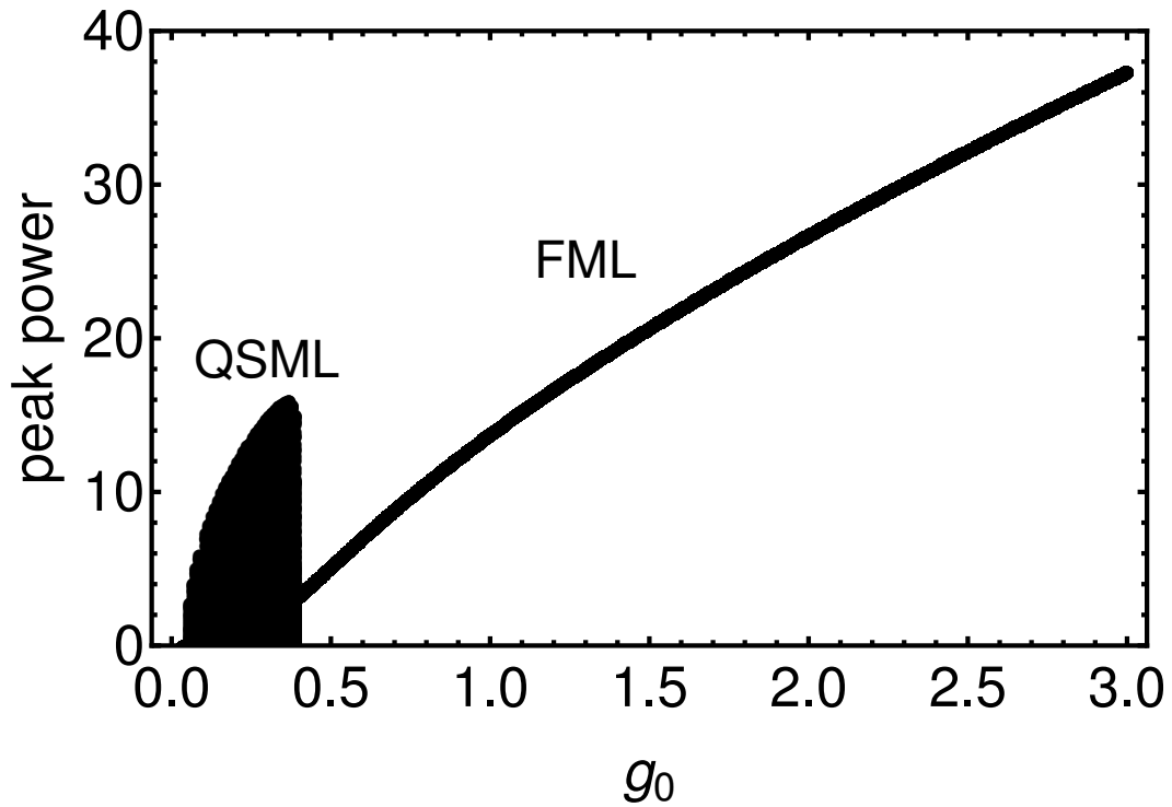
Figure 3: Bifurcation diagram similar to that shown in Fig. 1, but obtained with conventional class-B Haus model. QSML and FML denote Q-switched and fundamental mode-locking regimes, respectively. Parameter values are the same as in Fig. 1.
