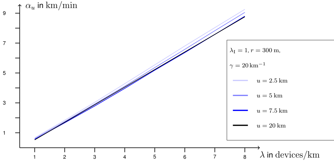
Figure 4: Simulations for the speed of malware propagation for the Markovian SI-model for growing observation windows as a function of \lambda .
