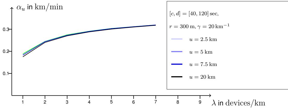
Figure 5: Simulations for the speed of malware propagation for the non-Markovian SI-model with uniform waiting times, for growing observation windows as a function of \lambda .
