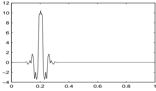
Figure 5.3.15: Dual generators \tilde{\phi}_{5,k} before and after biorthogonalization
