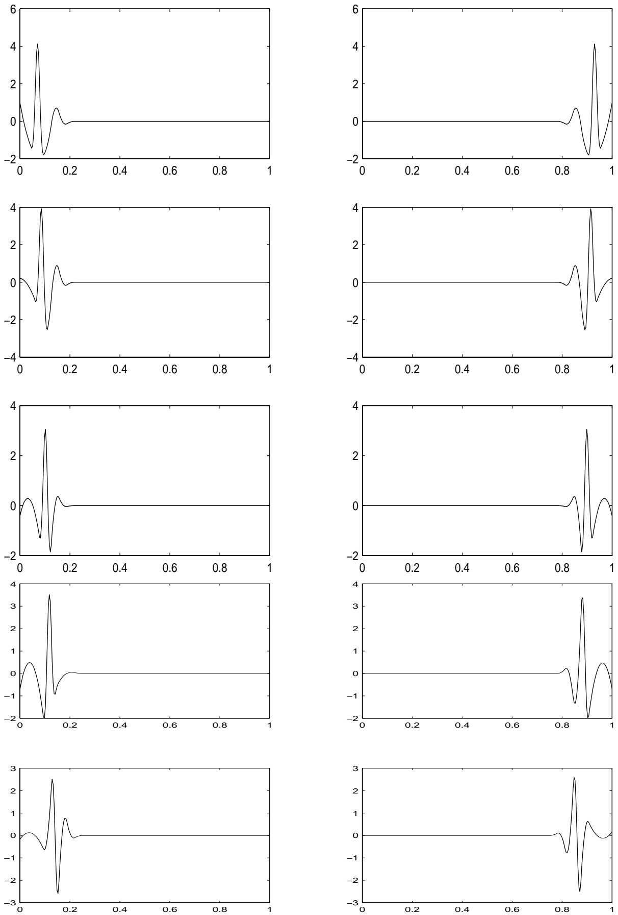
Figure 5.3.16: Primal wavelets \psi_{5,k} at left and right boundary
