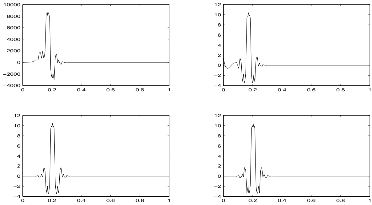
Figure 5.3.5: Dual generators \tilde{\phi}_{5,k} before and after biorthogonalization
