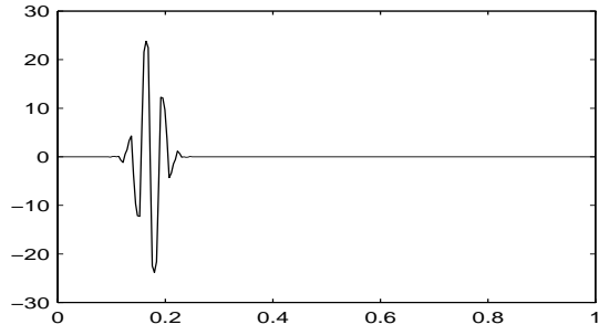
Figure 5.3.19: Dual wavelets \tilde{\psi}_{5,k} at left and right boundary
