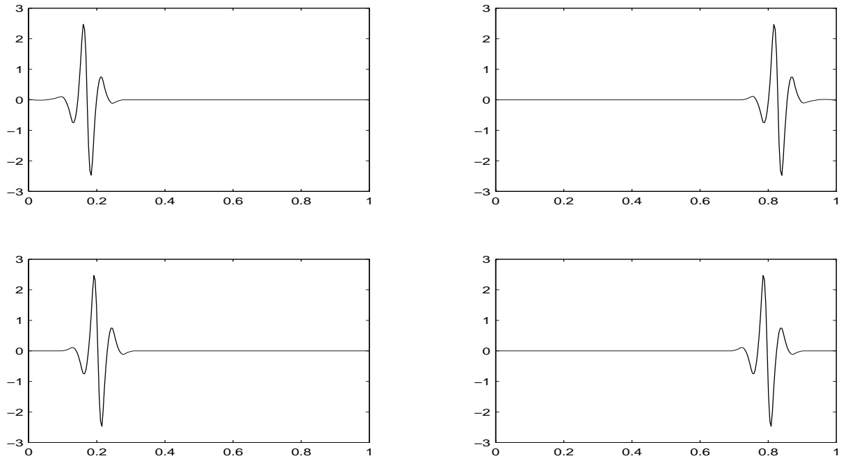
Figure 5.3.17: Primal wavelets \psi_{5,k} at left and right boundary
