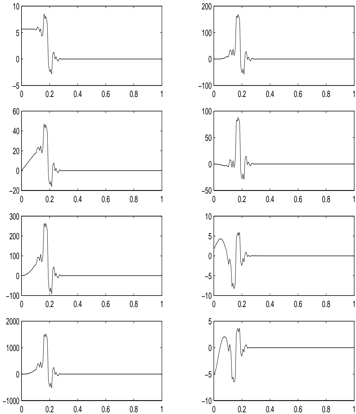
Figure 5.3.14: Dual generators \tilde{\phi}_{5,k} before and after biorthogonalization
