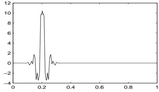
Figure 5.3.15: Dual generators \tilde{\phi}_{5,k} before and after biorthogonalization
