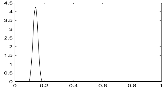
Figure 5.3.3: Primal generators \phi_{5,k}
