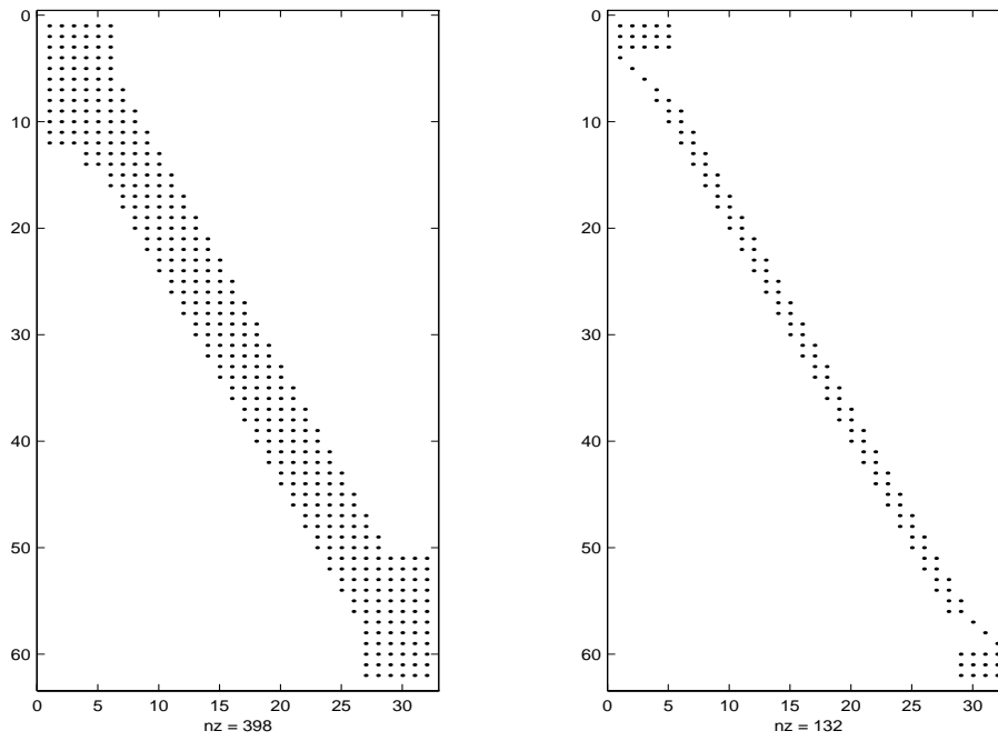
Figure 5.3.2: Nonzero pattern of refinement matrices M_{5,1} , \tilde{G}_{5,1}^T
