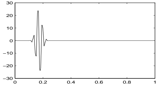
Figure 5.3.9: Dual wavelets \tilde{\psi}_{\varepsilon,k} at left and right boundary
