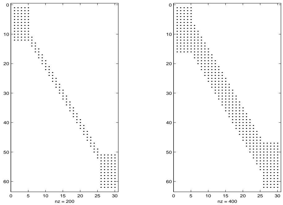
Figure 5.3.10: Nonzero pattern of refinement matrices M_{5,0}, \tilde{M}_{5,0}
