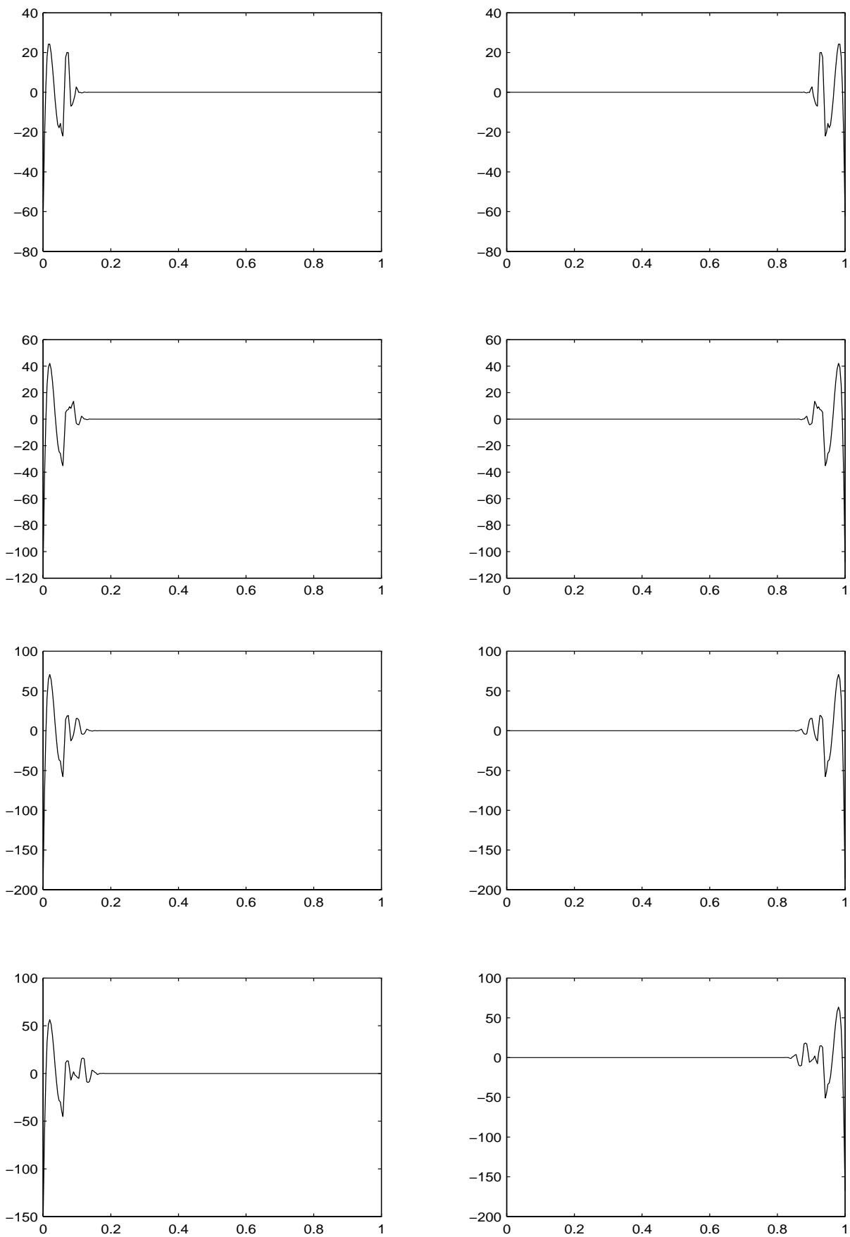
Figure 5.3.8: Dual wavelets \tilde{\psi}_{5,k} at left and right boundary
