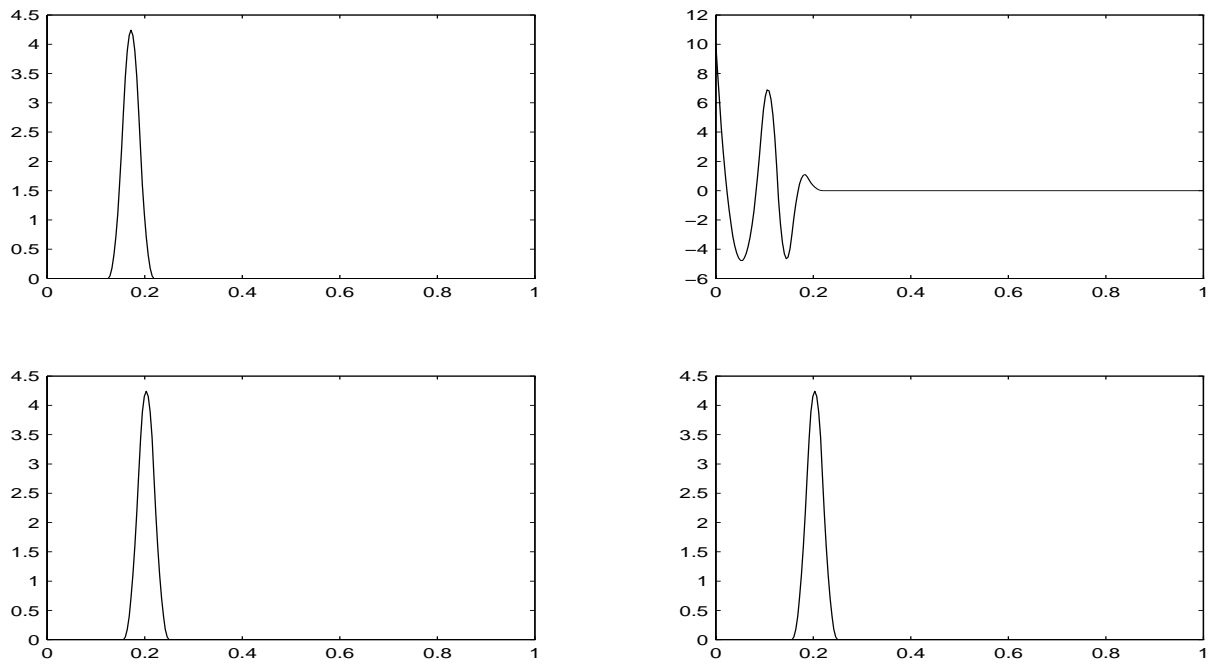
Figure 5.3.13: Primal generators \phi_{5,k} before and after biorthogonalization
