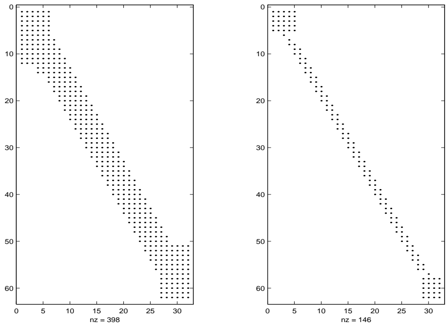
Figure 5.3.11: Nonzero pattern of refinement matrices M_{5,1}, \check{G}_{5,1}^T
