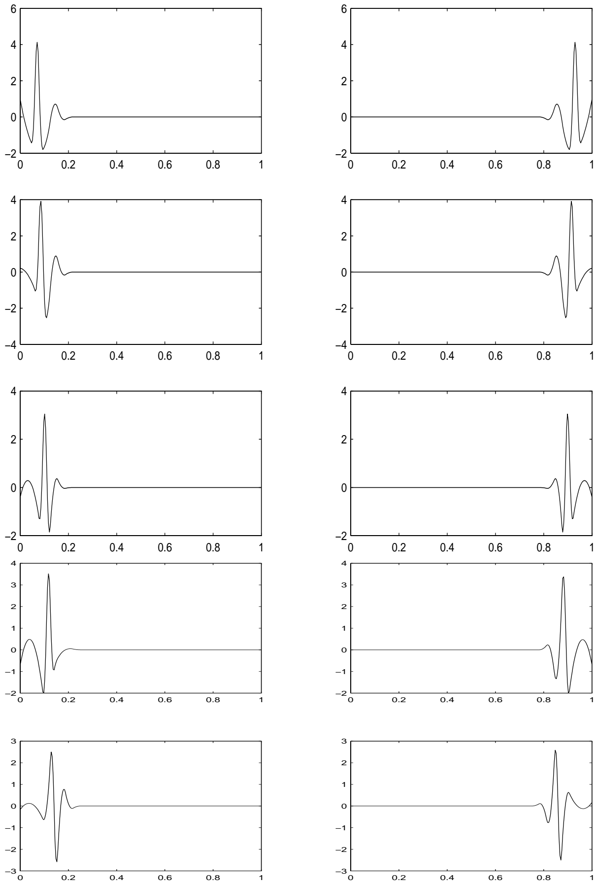
Figure 5.3.6: Primal wavelets \psi_{5,k} at left and right boundary
