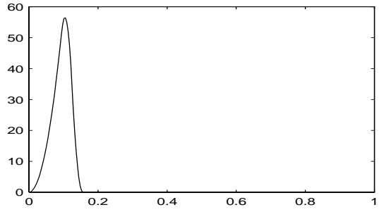
Figure 5.3.3: Primal generators \phi_{5,k}
