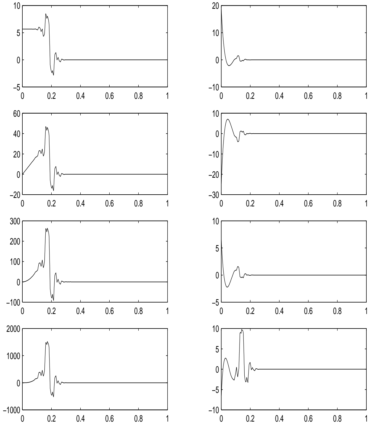
Figure 5.3.4: Dual generators \tilde{\phi}_{5,k} before and after biorthogonalization
