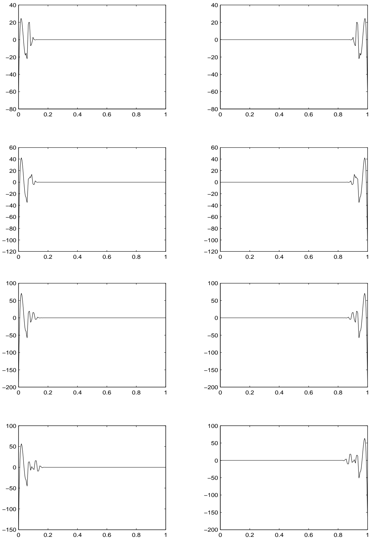
Figure 5.3.18: Dual wavelets \tilde{\psi}_{5,k} at left and right boundary
