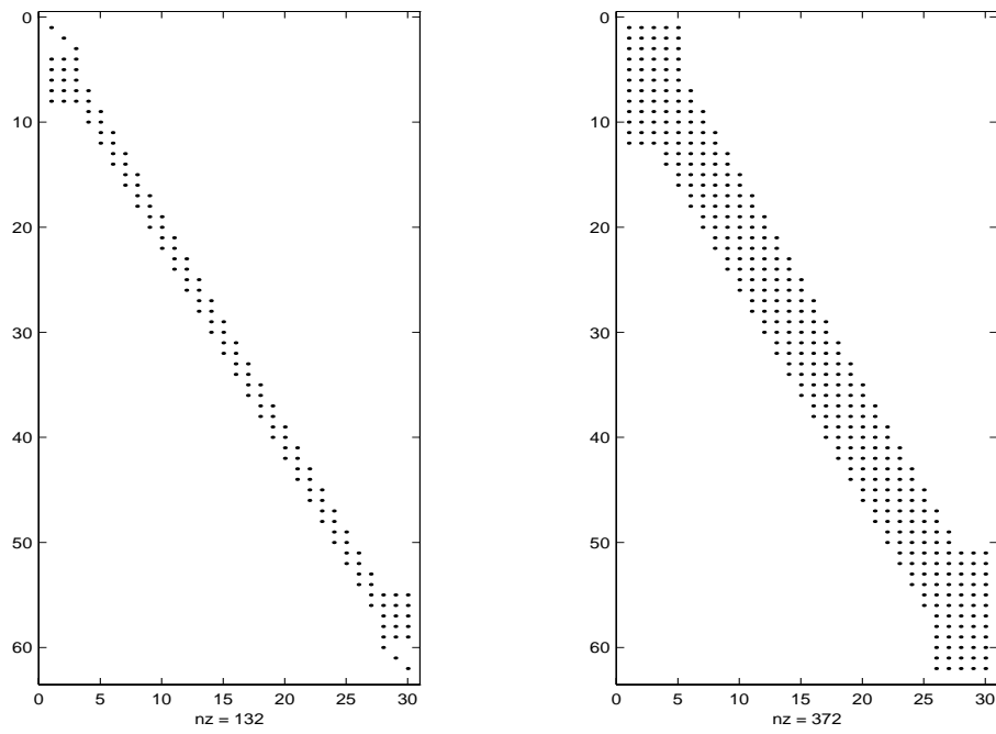
Figure 5.3.1: Nonzero pattern of refinement matrices M_{5,0}, \tilde{M}_{5,0}
