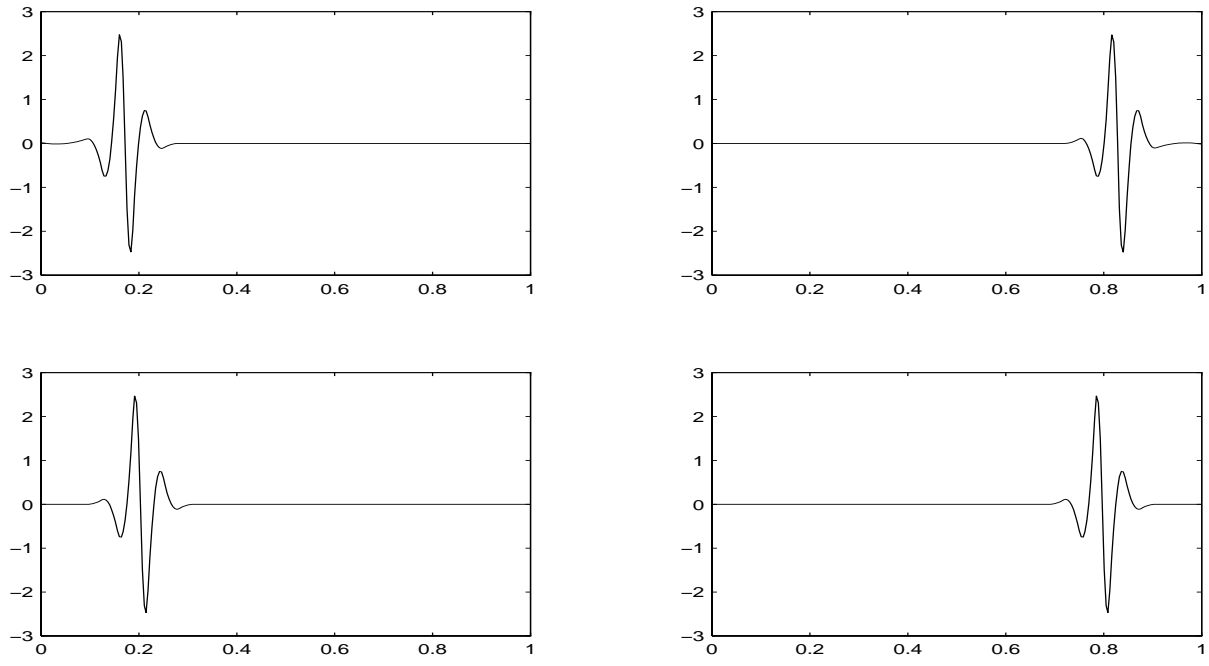
Figure 5.3.7: Primal wavelets \psi_{5,k} at left and right boundary
