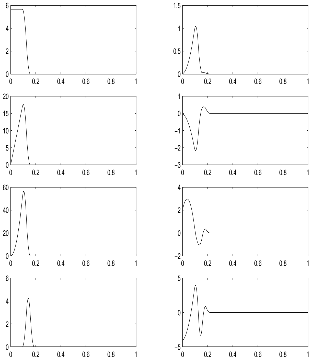
Figure 5.3.12: Primal generators \phi_{5,k} before and after biorthogonalization
