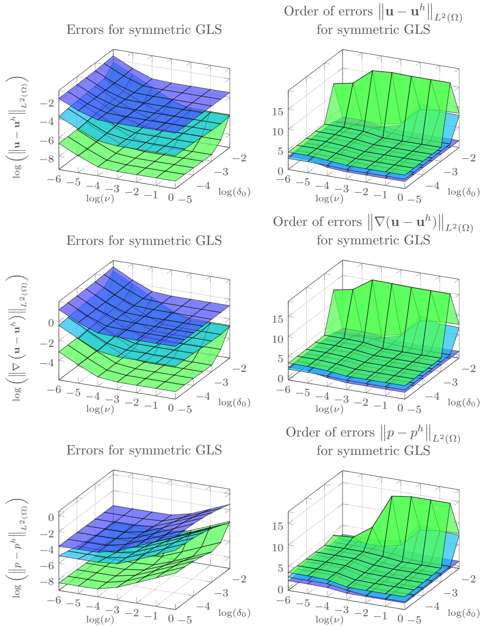
Figure 4: The errors (left) and computed orders of convergence (right) with respect to the L^2 (top) and H^1 semi-norm (middle) of the velocity, as well as the L^2 norm of the pressure (bottom) for the symmetric GLS method and P_1/P_1 (blue), P_2/P_2 (cyan), and P_3/P_3 (green).
