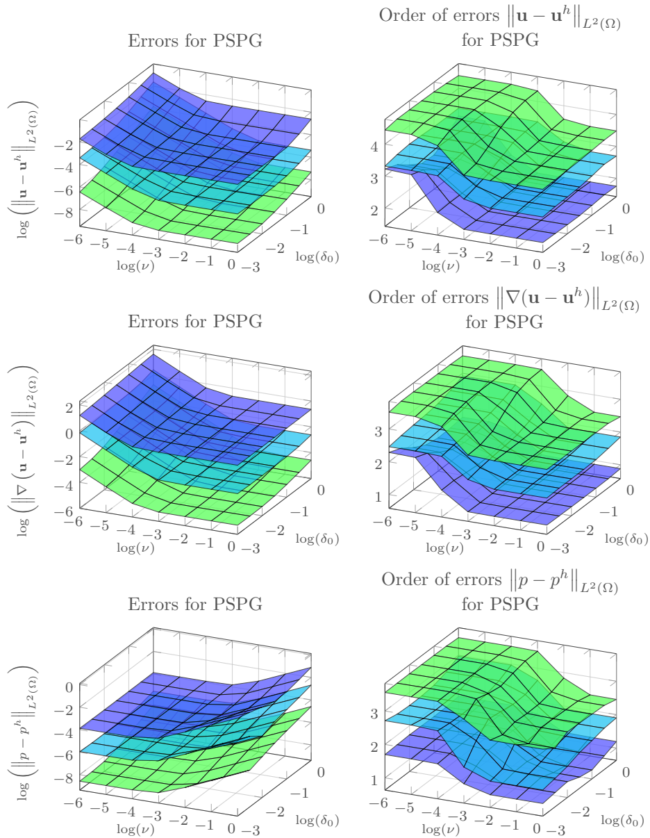
Figure 3: The errors (left) and computed orders of convergence (right) with respect to the L^2 (top) and H^1 semi-norm (middle) of the velocity, as well as the L^2 norm of the pressure (bottom) for the PSPG method and P_1/P_1 (blue), P_2/P_2 (cyan), and P_3/P_3 (green).
