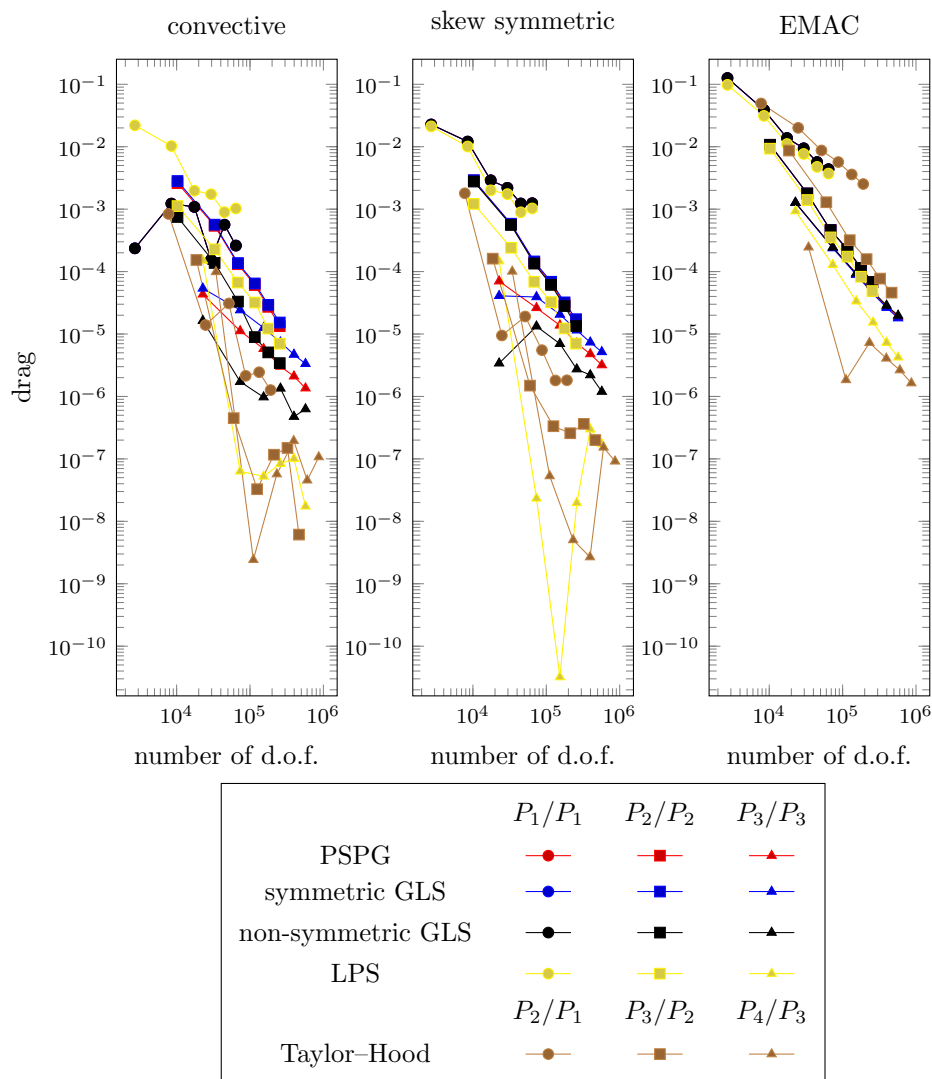
Figure 9: Computed absolute differences to reference value for drag using the convective (left), skew symmetric (center) and EMAC (right) nonlinear form on the unstructured grids, see Table 2 and Figure 8.
