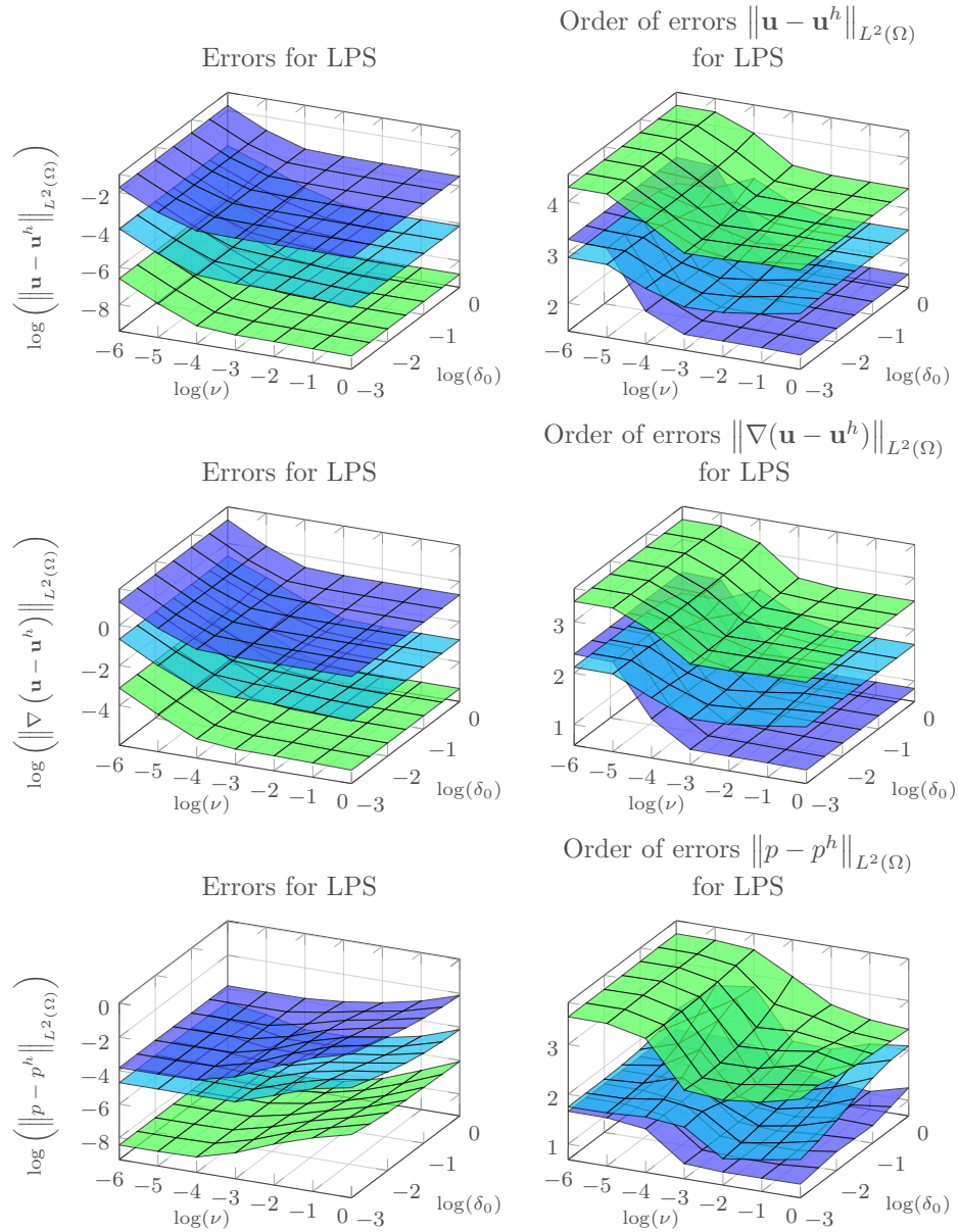
Figure 6: The errors (left) and computed orders of convergence (right) with respect to the L^2 (top) and H^1 semi-norm (middle) of the velocity, as well as the L^2 norm of the pressure (bottom) for the LPS method and P_1/P_1 (blue), P_2/P_2 (cyan), and P_3/P_3 (green).
