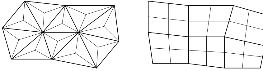
Figure 1: Relation between the meshes \mathcal{M}^h (bold lines) and \mathcal{T}^h (bold and fine lines) in the two-level method.
