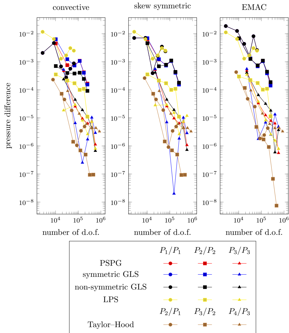
Figure 11: Computed absolute differences to reference value for the pressure difference at the cylinder using the convective (left), skew symmetric (center) and EMAC (right) nonlinear form on the unstructured grids, see Table 2 and Figure 8.
