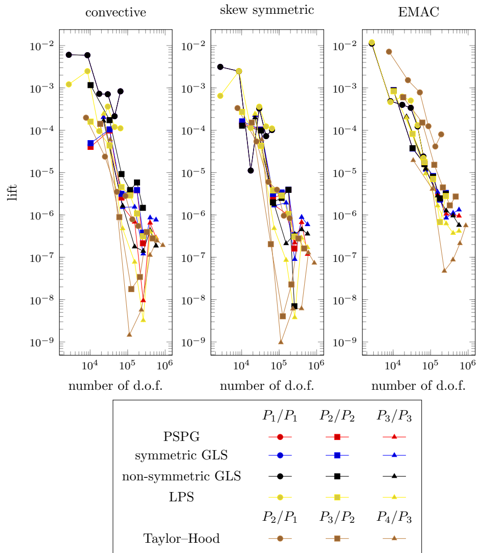
Figure 10: Computed absolute differences to reference value for lift using the convective (left), skew symmetric (center) and EMAC (right) nonlinear form on the unstructured grids, see Table 2 and Figure 8.
