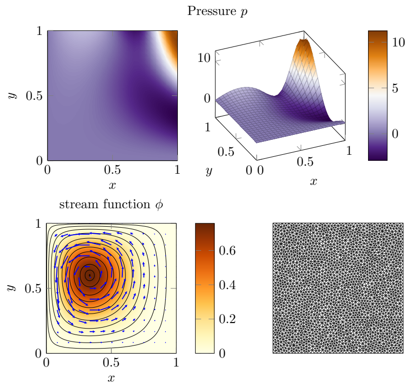
Figure 2: Visualizations of the solution of the Stokes example. Top: pressure p . Bottom left: stream function \phi together with streamlines and arrows of the velocity \mathbf{u} . Bottom right: For illustration, a generated grid which is coarser than the ones actually used.
