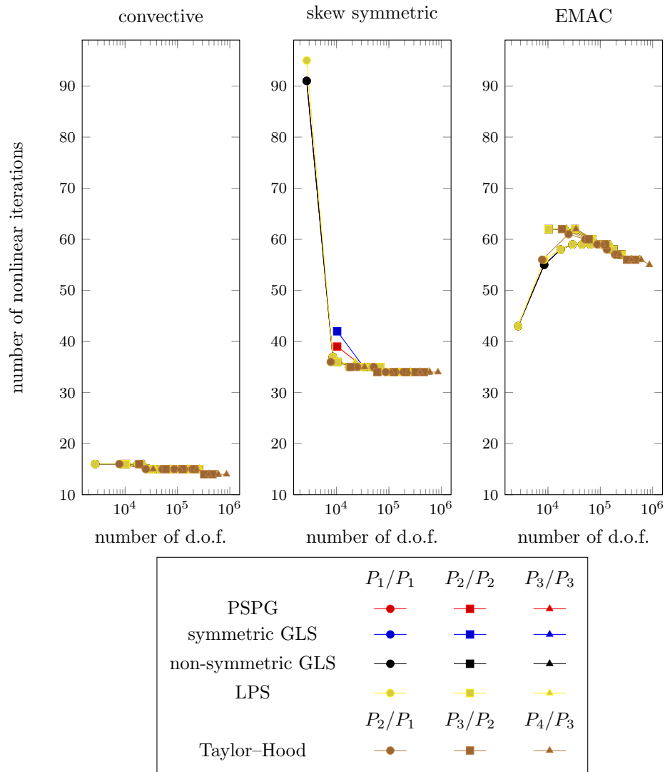
Figure 12: The number of nonlinear iterations needed using the convective (left), skew symmetric (center) and EMAC (right) nonlinear form on the unstructured grids, see Table 2 and Figure 8.
