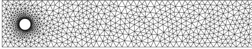
Figure 8: Coarse grid, generated with GMSH, used for the flow around a cylinder example.
