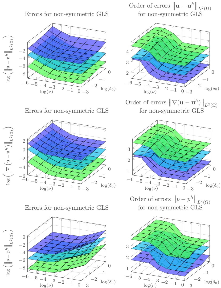
Figure 5: The errors (left) and computed orders of convergence (right) with respect to the L^2 (top) and H^1 semi-norm (middle) of the velocity, as well as the L^2 norm of the pressure (bottom) for the non-symmetric GLS method and P_1/P_1 (blue), P_2/P_2 (cyan), and P_3/P_3 (green).
