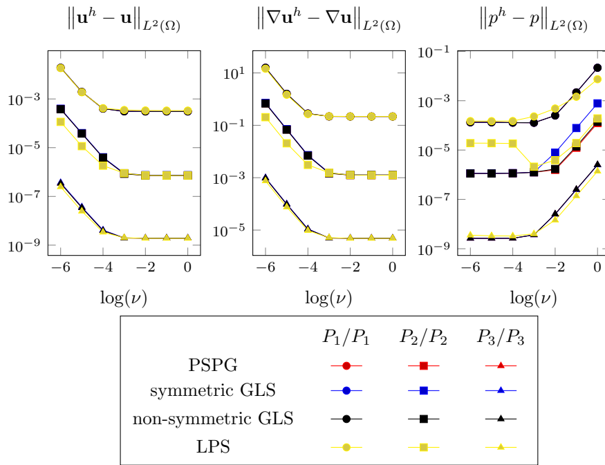
Figure 7: The L^2 -errors of the velocity (left), its gradient (middle) and of the pressure (right) for the considered methods and different polynomial degrees on the finest level 4. The stabilization parameter \delta_0 is always chosen such that the L^2 -error of the velocity is smallest among the used values for \delta_0 . Note that lines are often on top of each other, i. e., the methods led to very similar errors.
