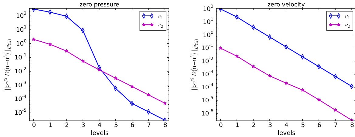
Figure 3: Errors \|\nu^{1/2}\mathbb{D}(\mathbf{u} - \mathbf{u}^h)\|_{L^2} for the special situations \alpha_v = 1, \alpha_p = 0 and \alpha_v = 0, \alpha_p = 1 .
