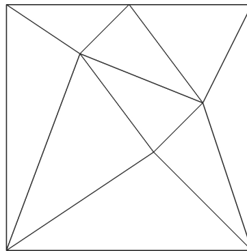
Figure 2: The coarsest grid, level 0.
