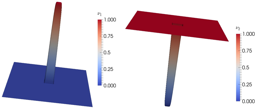
Figure 1: Viscosity functions \nu_1 and \nu_2 .
