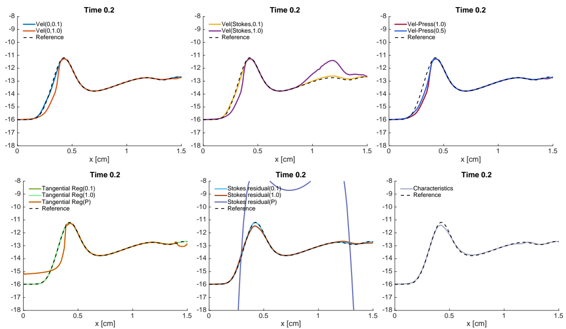
Figure 38: Benchmark 2 (stenosis), air regime (time t = 0.25 s): Pressure profiles along the open boundary [ \text{dyn/cm}^2 ].
