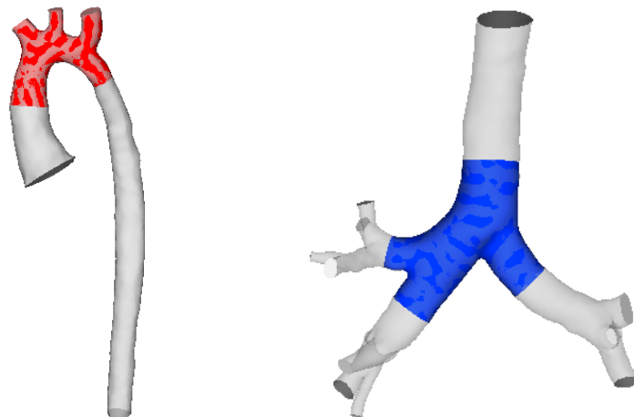
Figure 1: Illustration of the truncation of the computational domain (colored) from the originally segmented medical image (grey). Left: Aorta. Right: Airways.
