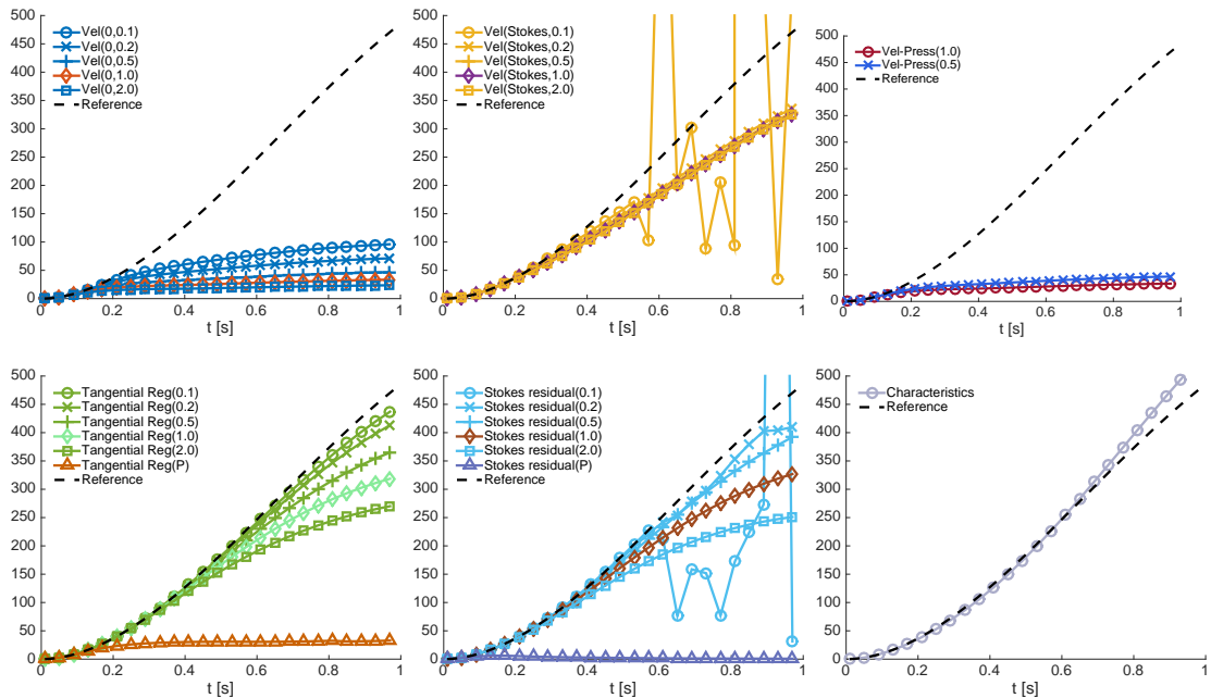
Figure 15: Benchmark 1 (full backflow), air regime, penalizing the tangential velocity on the open boundary: incoming flow rate [cm^2/s] over time [s] .
