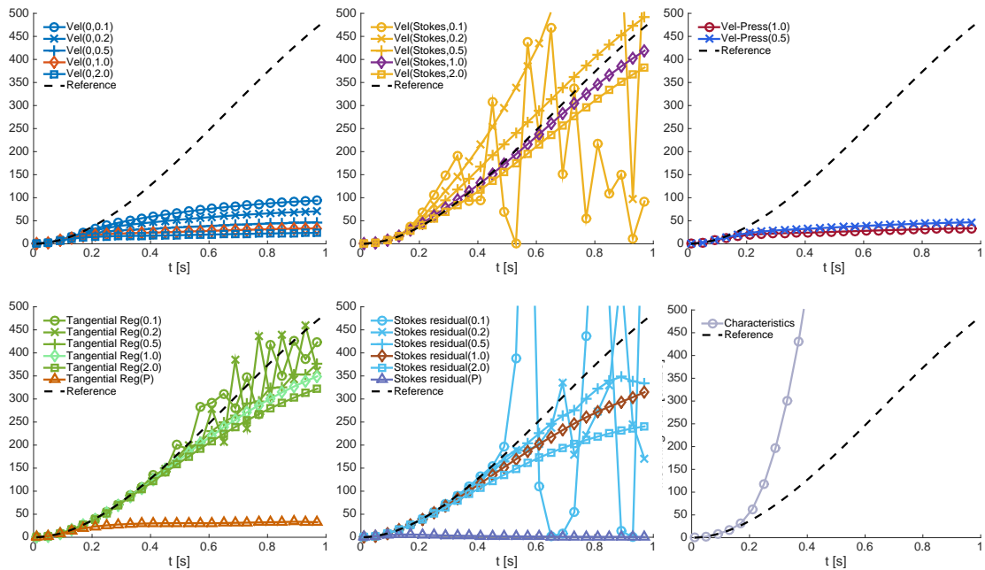
Figure 14: Benchmark 1 (full backflow), air regime: incoming flow rate [cm^2/s] over time [s] .
