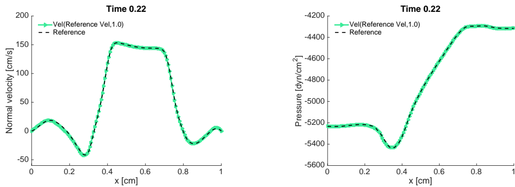
Figure 24: Benchmark 2 (stenosis), blood regime. Profiles of velocity at the open boundary (left) and pressure on the inlet boundary (right), using an open boundary stabilization based on a velocity penalization towards the reference velocity.
