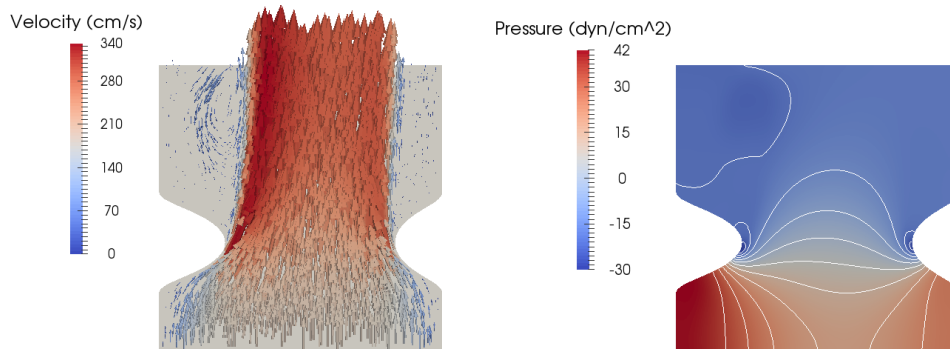
Figure 31: Benchmark 2 (stenosis), air regime. Reference solution at t=0.20 \text{ s} . Left: Mesh and glyph vector of the velocity field. Right: Pressure isolines.
