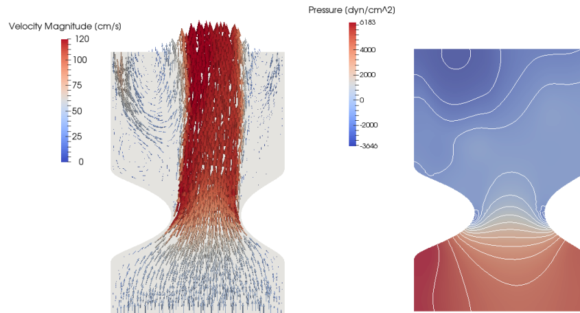
Figure 23: Benchmark 2 (stenosis), blood regime. Reference solution (computed in the domain \Omega_{\text{ext}} , but visualized only in \Omega ) at time t=0.15 s. Left: Glyph vector of the velocity field. Right: Pressure field, including isolines.
