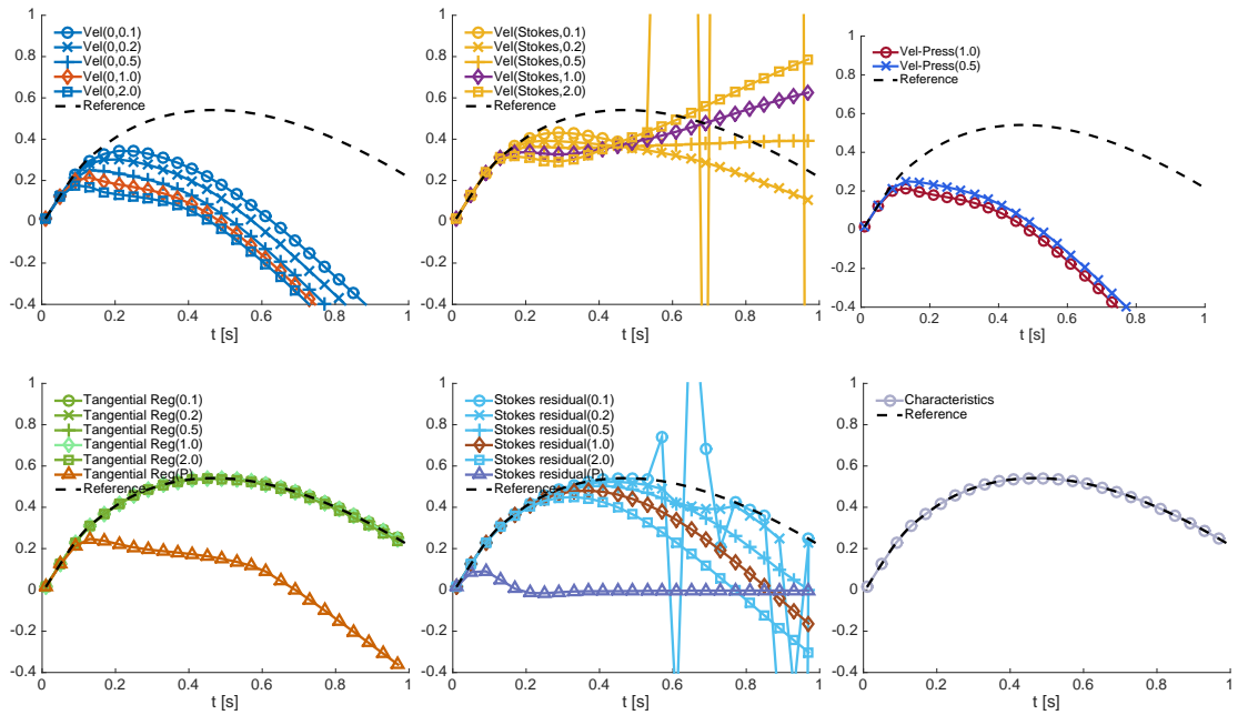
Figure 17: Benchmark 1 (full backflow), air regime, penalizing the tangential velocity on the open boundary: Average pressure drop [ \text{dyn/cm}^2 ] over time [s].
