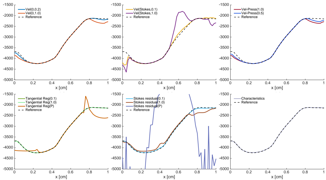
Figure 28: Benchmark 2 (stenosis), blood regime (time t = 0.17 s): Pressure profiles along the open boundary [dyn/cm 2 ].
