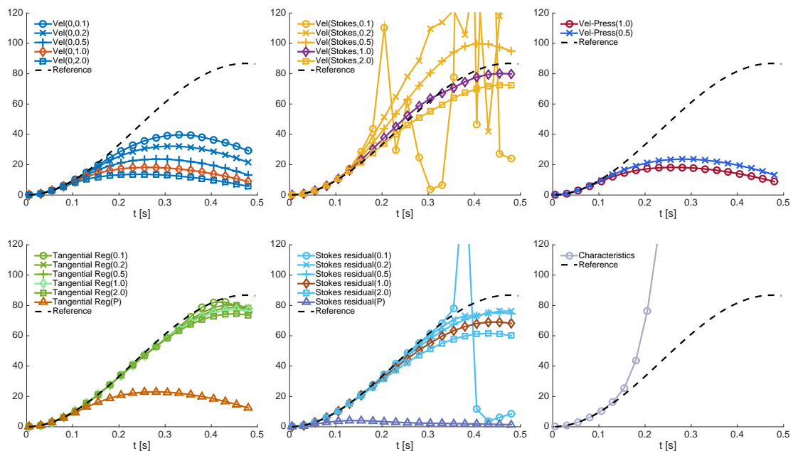
Figure 4: Benchmark 1 (full backflow), blood regime: incoming flow rate [cm 2 /s] over time [s].
