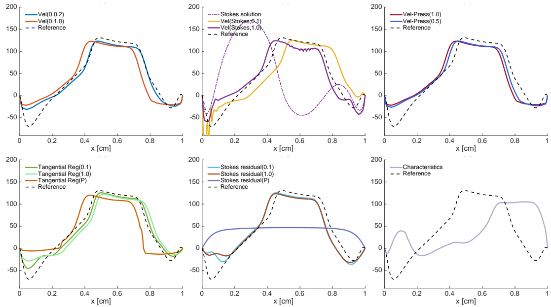
Figure 27: Benchmark 2 (stenosis), blood regime (time t = 0.17 s): Normal velocity profiles along the open boundary [cm/s].
