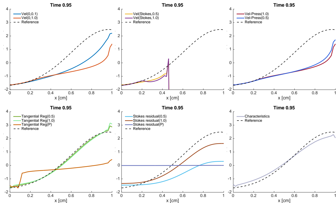
Figure 20: Benchmark 1 (full backflow), air regime (time t = 0.95 s): Pressure profiles along the open boundary [dyn/cm 2 ].
