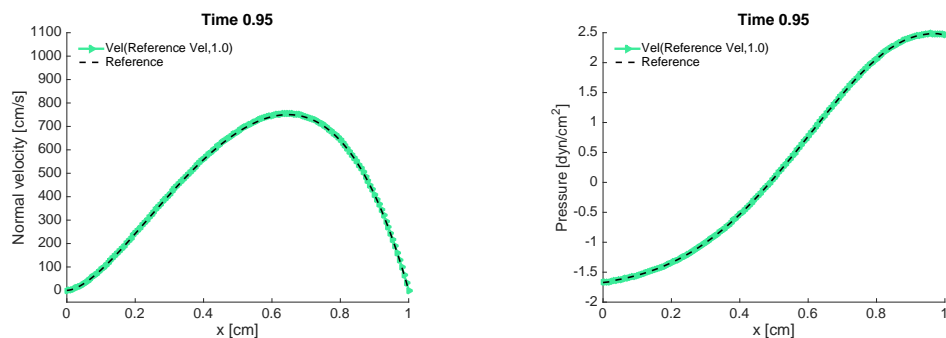
Figure 13: Profiles of velocity (left) and pressure (right) at the inflow boundary, using an open boundary stabilization based on a velocity penalization towards the reference velocity (Benchmark 1, air regime).
