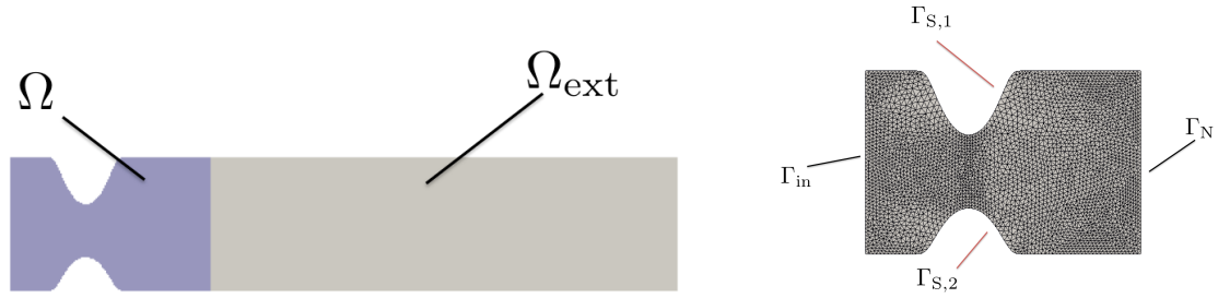
Figure 22: Left: The domains \Omega_{\text{ext}} and \Omega considered for this benchmark. Right: The shorter domain \Omega with the considered spatial discretization and the partition of the boundary.
