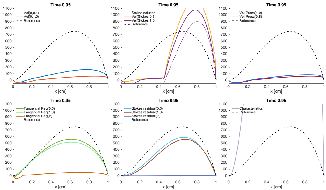
Figure 18: Benchmark 1 (full backflow), air regime (time t = 0.95 s): Normal velocity profiles along the open boundary [ \text{cm/s} ].
