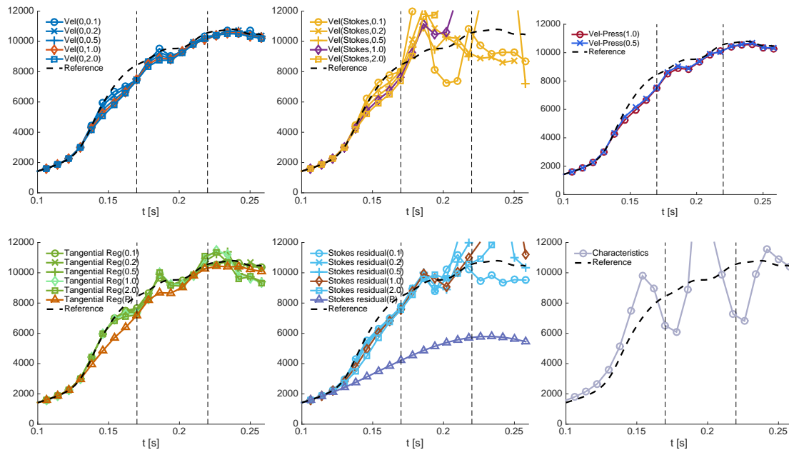
Figure 26: Benchmark 2 (stenosis), blood regime: Average pressure drop [dyn/cm 2 ] over time [s].
