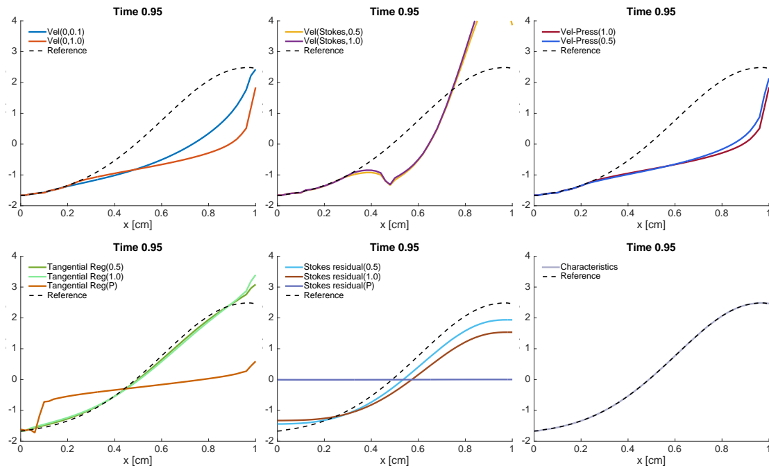
Figure 21: Benchmark 1 (full backflow), air regime, penalizing the tangential velocity on the open boundary (time t = 0.95 s): Pressure profiles along the open boundary [ \text{dyn}/\text{cm}^2 ].
