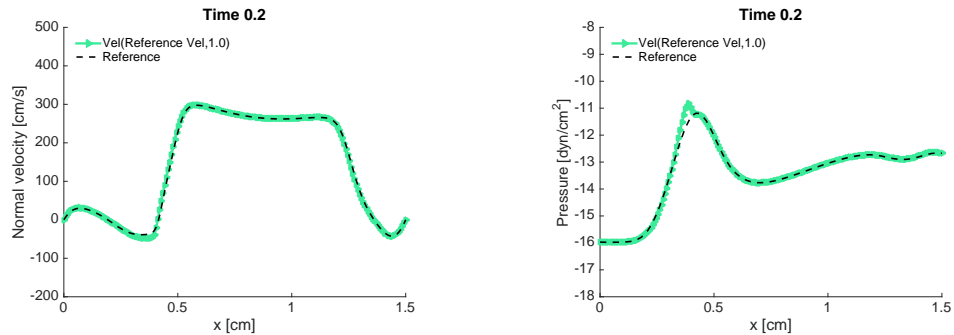
Figure 32: Profiles of velocity (left) and pressure (right) at the inflow boundary ( t = 0.20 \text{ s} ), using an open boundary stabilization consistent with the reference velocity (Benchmark 2, air regime).
