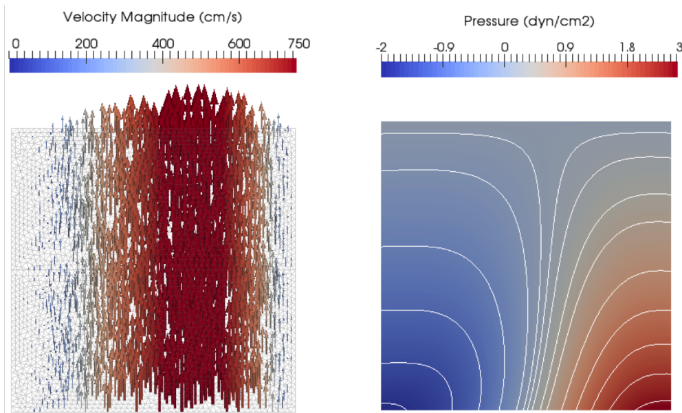
Figure 12: Reference solution (Benchmark 1, air) at peak backflow in air regime ( t=0.95 \text{ s} ). Left: Mesh and glyph vector of the velocity field. Right: Pressure isolines.
