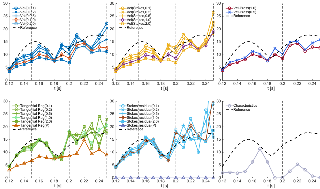
Figure 33: Benchmark 2 (stenosis), air regime: incoming flow rate [ \text{cm}^2/\text{s} ] over time [s].
