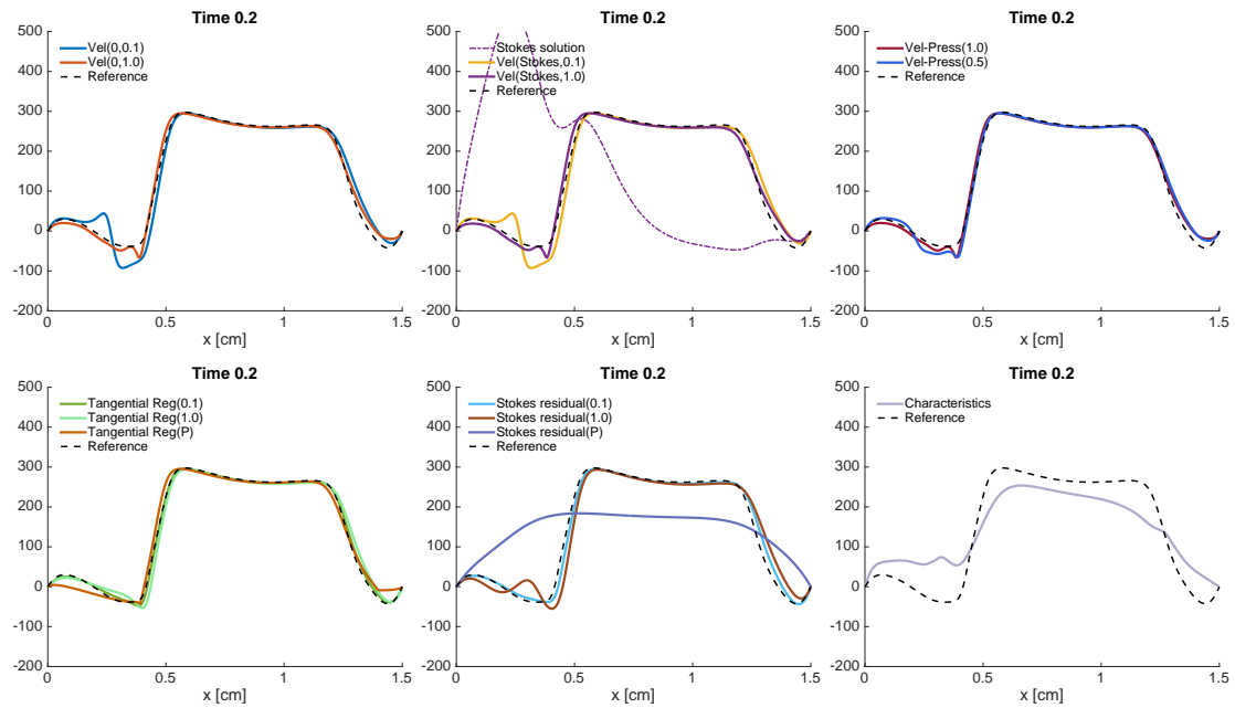
Figure 37: Benchmark 2 (stenosis), air regime (time t = 0.25 s): Normal velocity profiles along the open boundary [cm/s].
