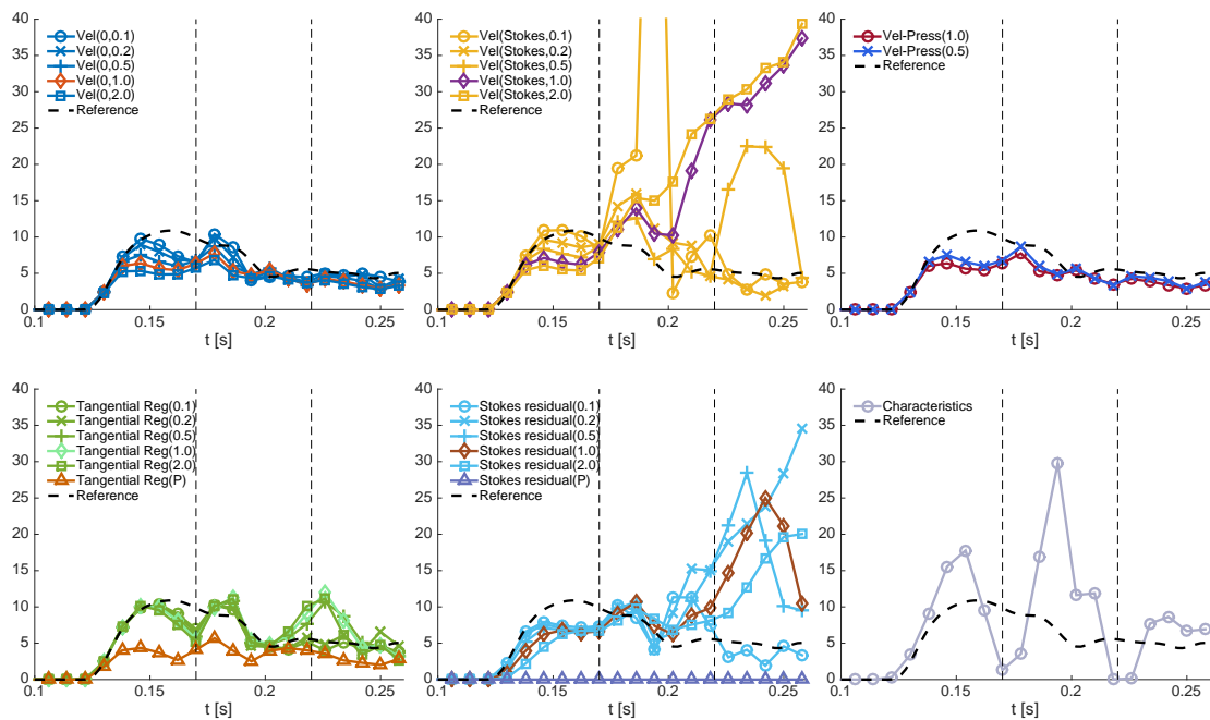
Figure 25: Benchmark 2 (stenosis), blood regime: incoming flow rate [\text{cm}^2/\text{s}] over time [\text{s}] .
