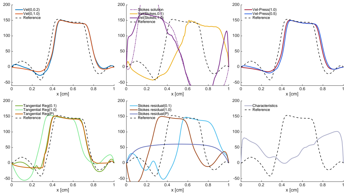
Figure 29: Benchmark 2 (stenosis), blood regime (time t = 0.22 s): Normal velocity profiles along the open boundary [cm/s].
