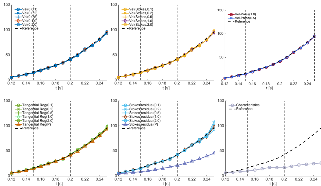
Figure 34: Benchmark 2 (stenosis), air regime: Average pressure drop [ \text{dyn}/\text{cm}^2 ] over time [s].
