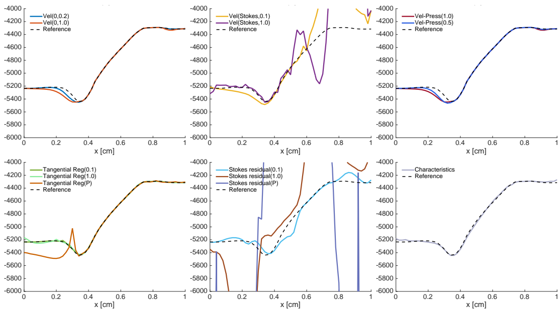
Figure 30: Benchmark 2 (stenosis), blood regime (time t = 0.22 s): Pressure profiles along the open boundary [dyn/cm 2 ].
