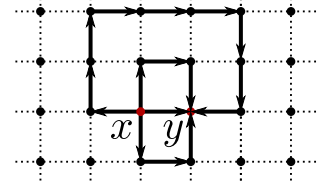
Figure 1: Independent paths
