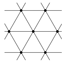
Figure 2: Triangular lattice.
