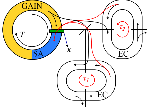
Figure 1: Schematic diagram of a two section ring cavity laser subject to optical feedback from two external cavities (EC). The yellow region represents the gain section, the blue region corresponds to the saturable absorber (SA) section and the green bar indicates the spectral filtering element.
