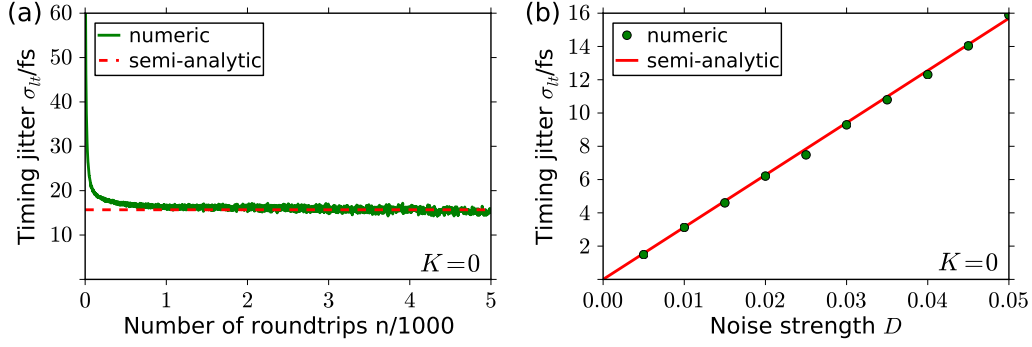
Figure 2: (a) Comparison of the results of numerical calculation of pulse timing jitter (green solid line), obtained for different numbers of round-trips n , with the timing jitter value from formula (8) (red dashed line). (b) Estimation of timing jitter, calculated using formula (8) (red solid line) and the numerical method (green dots), vs noise strength D . Parameters: K = 0 , \tau = 0 , T = 25 ps, \kappa = 0.3 , \gamma^{-1} = 125 fs, \gamma_g^{-1} = 500 ps, \gamma_q^{-1} = 5 ps, s = 10 , q_0^{-1} = 10 ps, g_0^{-1} = 250 ps, \alpha_g = 2 , \alpha_q = 1 .
