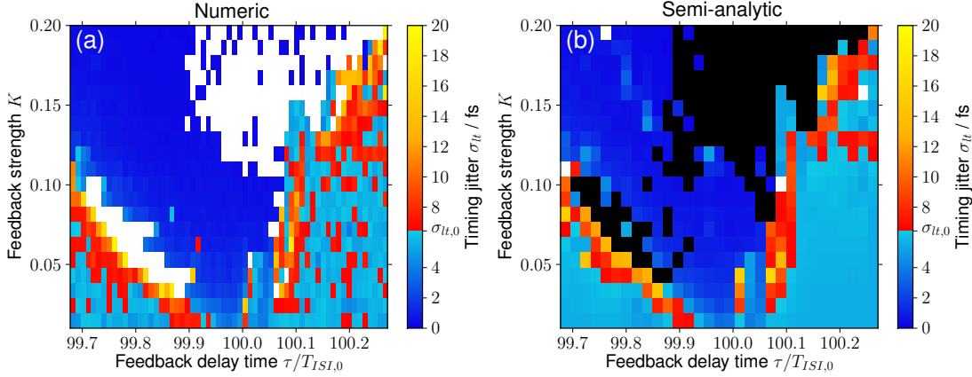
Figure 4: Timing jitter in dependence of the feedback cavity delay time and feedback strength, calculated numerically (a) and using the semi-analytical method (b). The timing jitter is indicated by the colour code and \sigma_{tt,0} is the timing jitter of the solitary laser. Regions in white indicate a timing jitter greater than 20fs. In subplot (b) black marks the regions where the deterministic system has a non-periodic solution and the semi-analytical method cannot be applied. Parameters: D = 0.2 , \alpha_g = 2 , \alpha_q = 1.5 , others are as in table 1.
