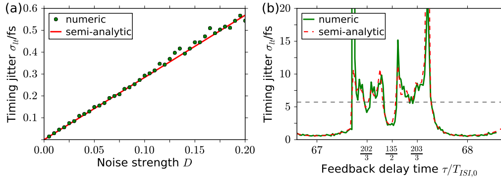
Figure 3: (a) Timing jitter in dependence of the noise strength, calculated using the semi-analytic method (red line) and the numerical method described in [OTT14b] (green dots) for \tau = 70T_{ISI,0} . (b) Timing jitter in dependence of the feedback delay time, calculated using the semi-analytic method (red dashed line) and the numerical method (green line) for D = 0.2 . Parameters: \alpha_g = 0 , \alpha_q = 0 , K = 0.1 . Other parameters are as in Table 1.
