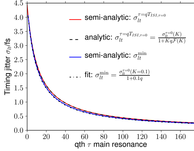
Figure 6: Timing jitter \sigma_{lt} at the exact main resonances (red solid line) and the minimum timing jitter in each resonance region (blue solid line) as a function of the number q of the main resonance, calculated using the semi-analytic method. The dashed line shows the timing jitter at the exact main resonances given by the analytic expression Eq. (13). The dot-dashed line shows the fit of Eq. (14) to the minimum timing jitter in each resonance regions. Parameters: K = 0.1 , D = 0.2 , \alpha_g = 0 , \alpha_q = 0 , others as in table 1.
