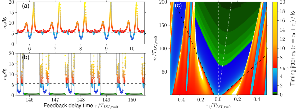
Figure 5: (a) and (b) Timing jitter \sigma_{lt} in dependence of the feedback cavity delay time. The colour code indicates the timing jitter according to the colour bar given in subplot (c). The black dashed line indicates the timing jitter of the solitary laser. (c) Timing jitter \sigma_{lt} in dependence of the feedback cavity delay time, where \tau = \tau_0 + \tau_1 for any given point. The horizontal axis spans one T_{ISI,\tau=0} and is centered on an exact main resonance. The vertical axis indicates the number of the main resonance. The timing jitter is indicated by the colour code and \sigma_{lt,0} is the timing jitter of the solitary laser. Parameters: K = 0.1 , D = 0.2 , \alpha_g = 0 , \alpha_q = 0 , others as in table 1.
