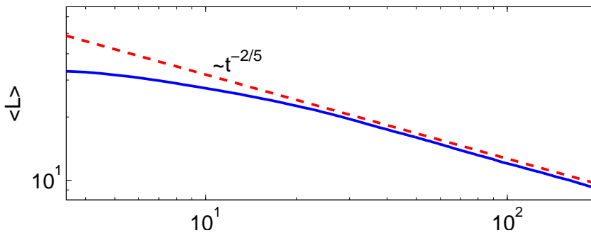
Figure 3: Coarsening diagram for the wavelet-Allen–Cahn equation, using the same parameters as in Figure 2. The diagram shows the average length scale \langle L \rangle , versus t as a solid line, where \langle L \rangle is defined in (38).
