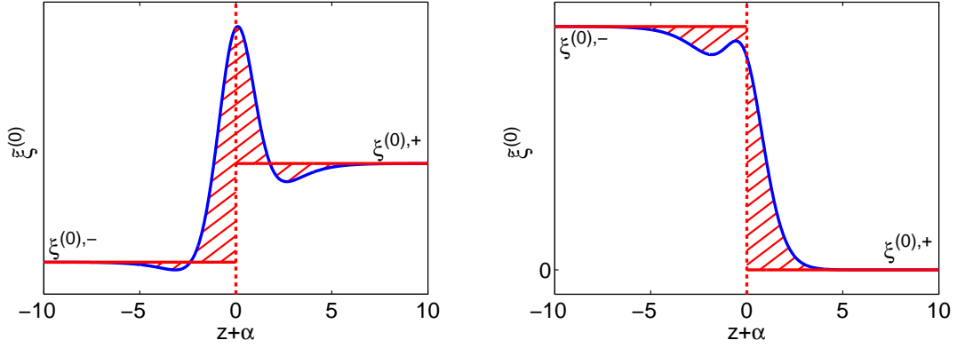
Figure 2: Blue: \tilde{\xi}^{(0)} , Shaded areas indicate \xi_I^{(1)} , Left: \gamma = 10 and c_0/\dot{x}_I^{(0)} = -0.4 Right: \gamma = 10 and c_0/\dot{x}_I^{(0)} = -1
