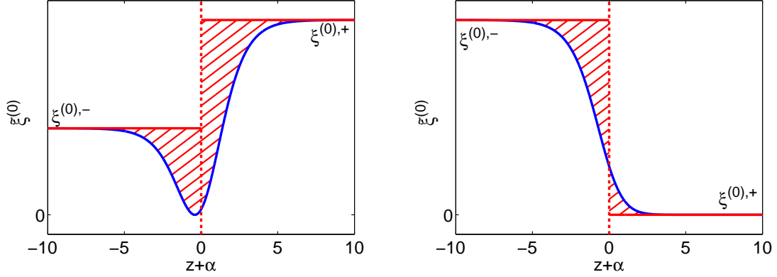
Figure 1: Blue: \tilde{\xi}^{(0)} , Shaded areas indicate \xi_I^{(1)} , Left: \gamma = 0 and c_0/\dot{x}_I^{(0)} = -0.4 Right: \gamma = 0 and c_0/\dot{x}_I^{(0)} = -1
