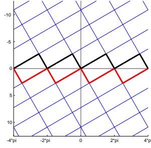
Figure 1: \mathcal{D}_2(\theta, k_p) with \theta = -\frac{\pi}{6} , k_p = 2 .
