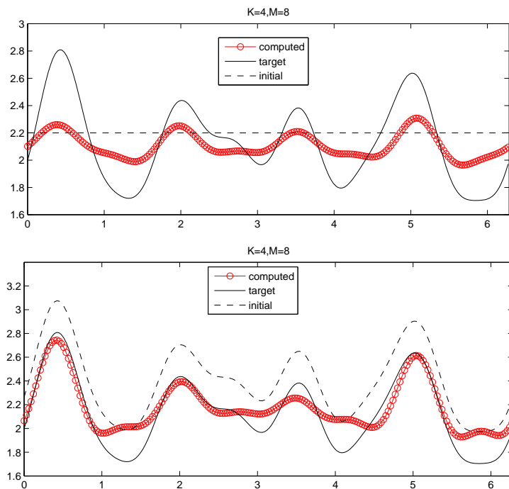
Figure 5: Example 2. K=4, M=8, \delta = 0 .
