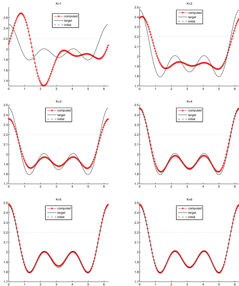
Figure 3: Sensitivity of the method to the parameter K in Example 1.
