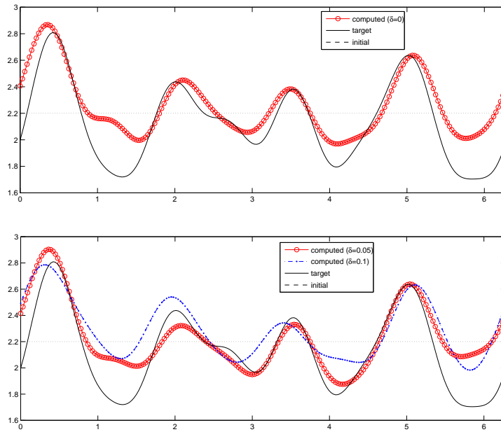
Figure 4: Example 2. K=7, M=8 .
