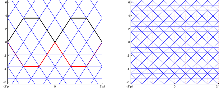
Figure 2: Left: \mathcal{N}_3(\theta, k_p) with \theta = -\frac{\pi}{6} , k_p = 2 . Right: \mathcal{N}_4(0, k_p) with k_p = 4 .
