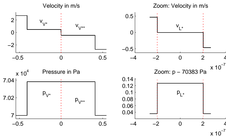
Figure 14: Example 3, condensation by compression
