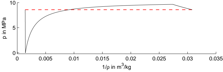
Figure 2: Equation of state: p(1/\rho) for T_0 = 573.15K , dashed red: Maxwell line
