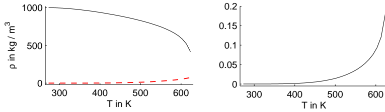
Figure 3: a) dashed red: \tilde{\rho}(T) , black: \rho_m(T) b) \tilde{\rho}(T)/\rho_m(T)
