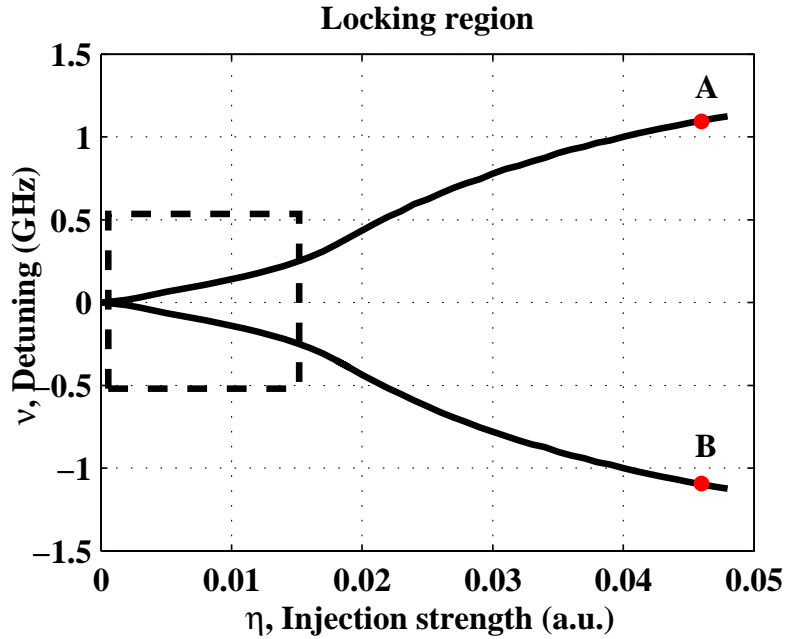
Figure 4: Locking cone for injections of small intensity with the frequency close to the central mode of the mode locked regime for \alpha_g = \alpha_q = 0 , g_0 = 1.0 , q_0 = 2.0 , \kappa = 0.3 , s = 10.0 , \gamma = 15.0 , \gamma_g = 0.01 , \gamma_q = 1.0 , T = 2.5 .
