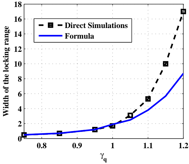
Figure 5: Dependence of the width of the locking cone on \gamma_q . T = 2.5 , \gamma = 30 , \kappa = 0.1 , g_0 = 1 , q_0 = 2 , \gamma_g = 0.01 , s = 25 .
