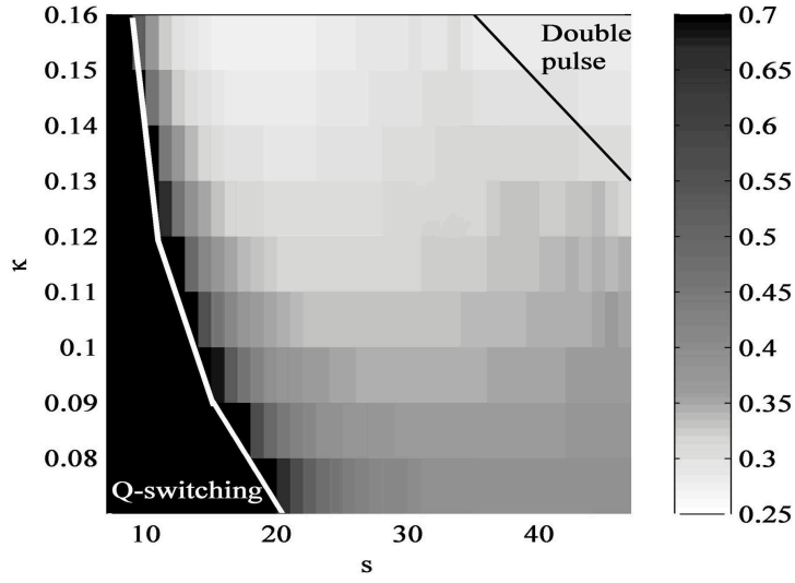
Figure 8: Dependence of the width of the locking cone on \kappa and s . T = 2.5 , \gamma = 30 , g_0 = 1 , q_0 = 2 , \gamma_g = 0.01 .
