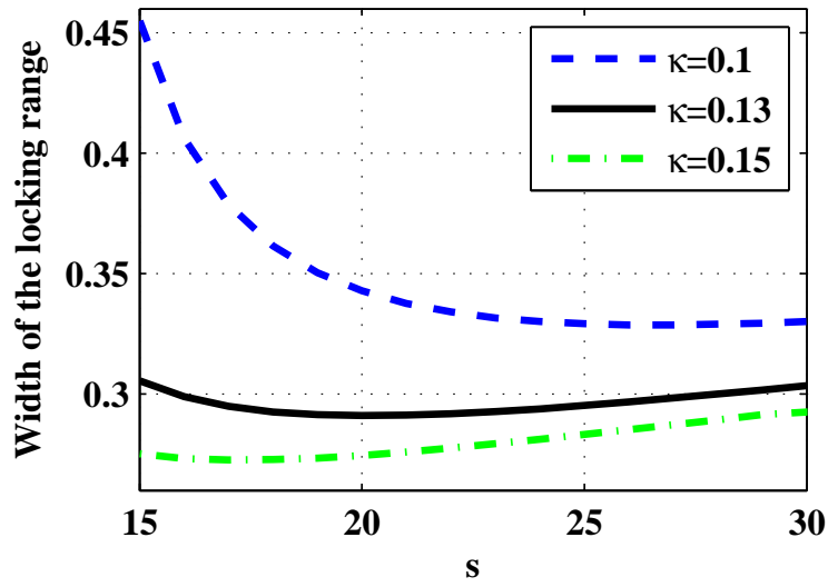
Figure 9: Dependence of the width of the locking cone on s . T = 2.5 , \gamma = 30 , g_0 = 1 , q_0 = 2 , \gamma_g = 0.01 .
