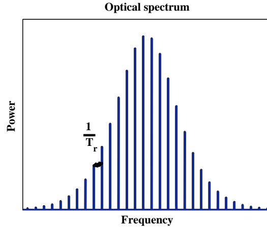
Figure 1: Frequency comb of the output of the mode locked laser.
