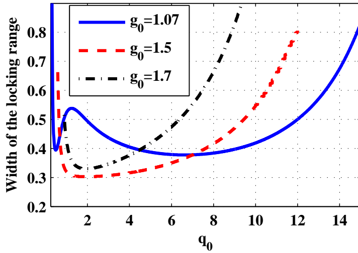
Figure 7: Dependence of the width of the locking cone on q_0 . T = 2.5 , \gamma = 30 , \kappa = 0.1 , q_0 = 4 , \gamma_g = 0.01 , s = 25 .
