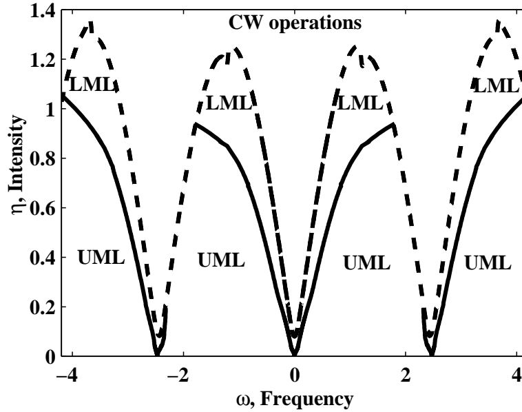
Figure 2: Locking regions for \alpha_g = \alpha_q = 0 , g_0 = 1.0 , q_0 = 2.0 , \kappa = 0.3 , s = 10.0 , \gamma = 15.0 , \gamma_g = 0.01 , \gamma_q = 1.0 , T = 2.5 .
