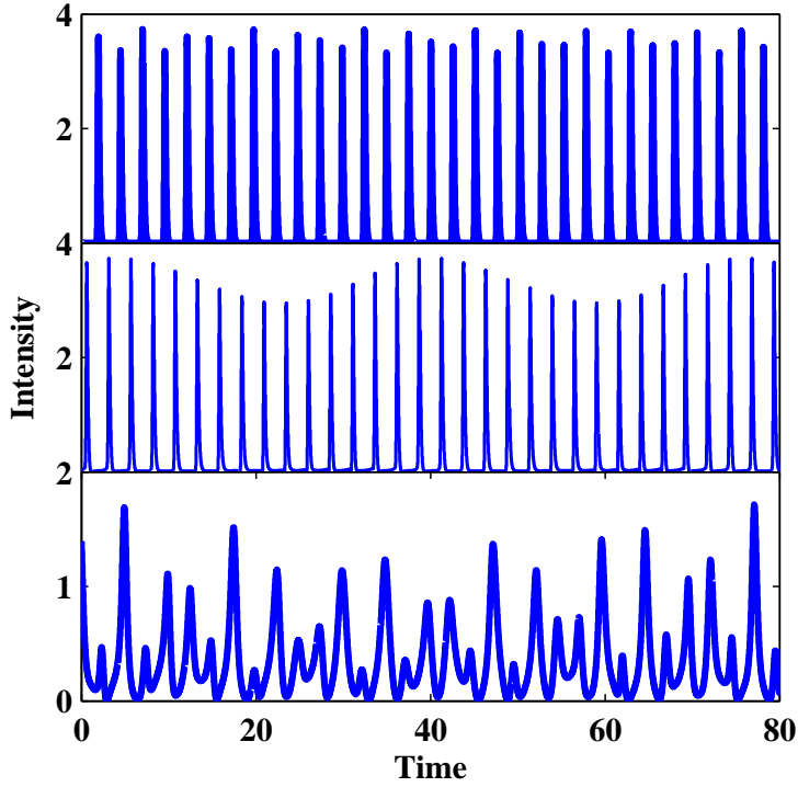
Figure 3: Time traces of unlocked ML (UML) solutions. \alpha_g = \alpha_q = 0 , g_0 = 1.0 , q_0 = 2.0 , \kappa = 0.3 , s = 10.0 , \gamma = 15.0 , \gamma_g = 0.01 , \gamma_q = 1.0 , T = 2.5 .
