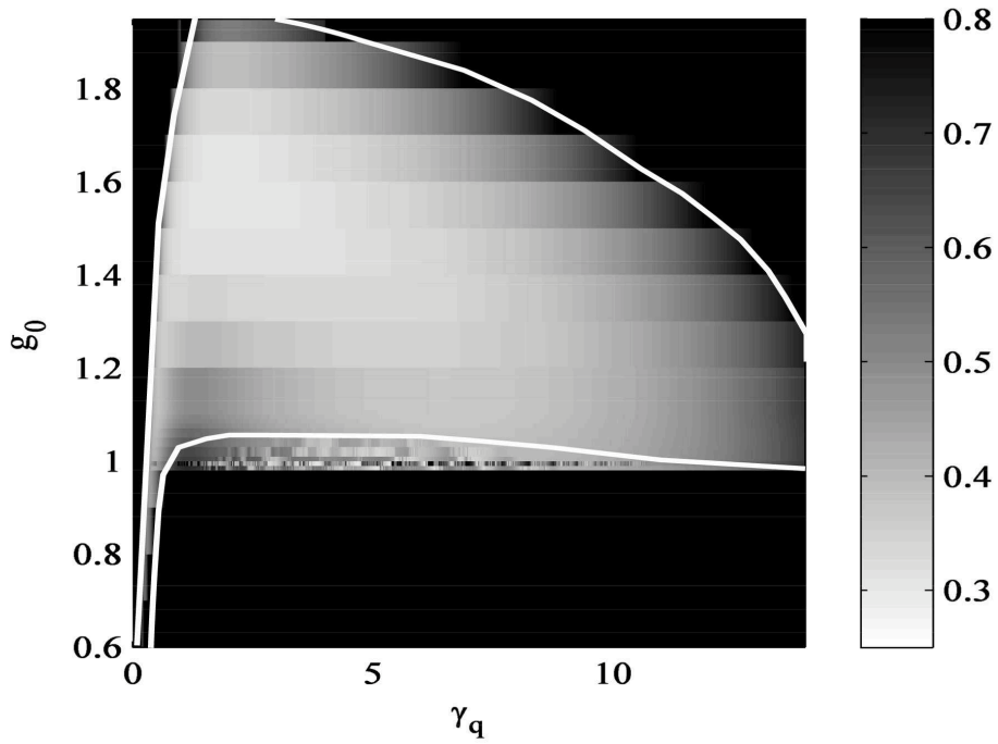
Figure 6: Dependence of the width of the locking cone on \gamma_q and g_0 . T = 2.5 , \gamma = 30 , \kappa = 0.1 , q_0 = 4 , \gamma_g = 0.01 , s = 25 .
