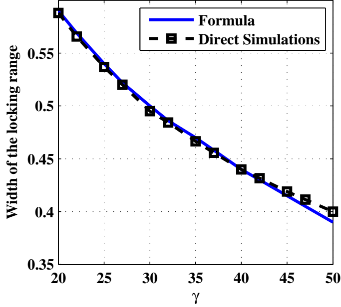
Figure 10: Dependence of the width of the locking cone on \gamma . T = 2.5 , \kappa = 0.1 , g_0 = 1 , q_0 = 2 , \gamma_g = 0.01 , \gamma_q = 0.75 , s = 25 .
