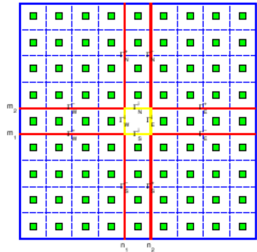
Fig. (29): A bi-periodic potential function with a defect in the center.
