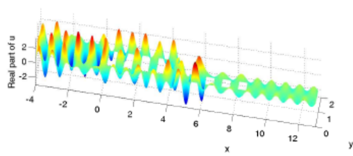
Fig. (25): Real part of the wave function for k = 8 .
