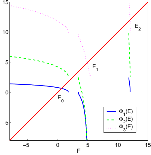
Fig. (9): The first three branches of \Phi(E) being restricted to [-8, 15] : E_0 = 6.42647(-1) . E_1 = 4.88651 . E_2 = 1.20164(1) .
