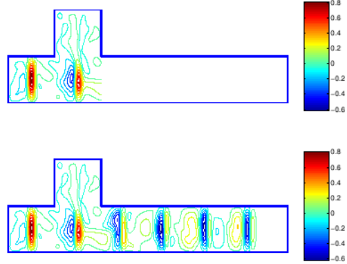
Fig. (13): Solutions at time t = 6 . The number of modes is 10. The reference solution is obtained by taking \Delta x = \Delta z = 0.00125 and \Delta t = 0.000625 .
