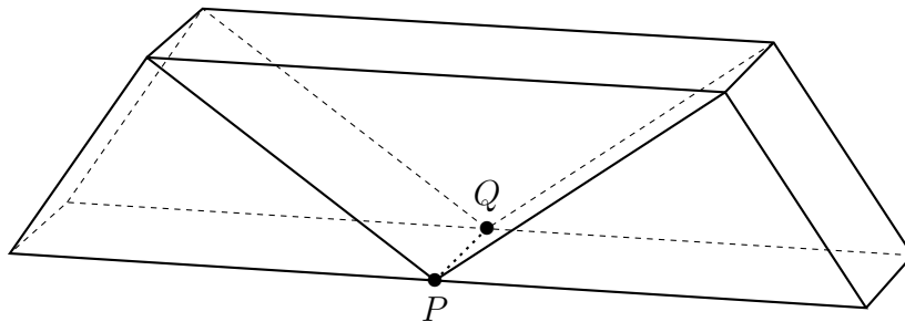
Figure 1: Direct vision prism composed of crown and flint glass (double Amici prism). At the three-material edge \overline{PQ} optical crown, flint, and again crown meet.
