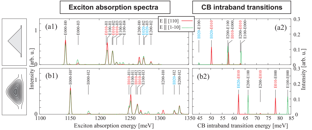
Figure 18: (Color online) Excitonic absorption spectra (left panel) and CB intraband transition spectra (right panel) shown for the unannealed and the strongest annealed QD of series G . First and second order piezoelectric effects are included.
