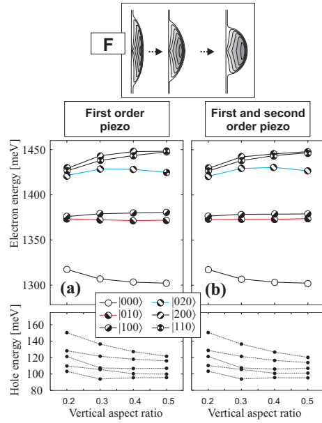
Figure 13: (Color online) Single-particle electron and hole energies for series F versus the vertical aspect ratio ar_V . In the left panel (a) the first order piezoelectric effect is accounted for using the experimental value of \epsilon_{14} only, whereas for the right hand panel also the second order is taken into account, using the piezoelectric constants from Ref. [11].
