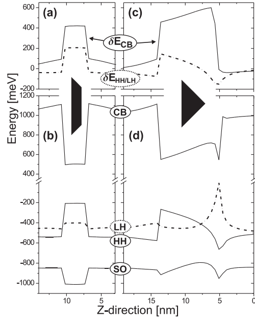
Figure 3: Impact of strain on the local band edges for the cases of a full and a truncated pyramid. (a) and (c): The dotted lines indicate the energy shift of the VB imposed by biaxial strain: \delta E_{HH/LH} = b/2 \epsilon_b(\mathbf{r}) . The solid line marks the contribution of the hydrostatic strain \delta E_c = a_c \epsilon_h(\mathbf{r}) . The resulting local band edge positions are shown in panels (b) and (d). While the HH-band inside the truncated QD is always above the LH-band, a crossing between HH and LH band edge occurs in the full pyramid (d).
