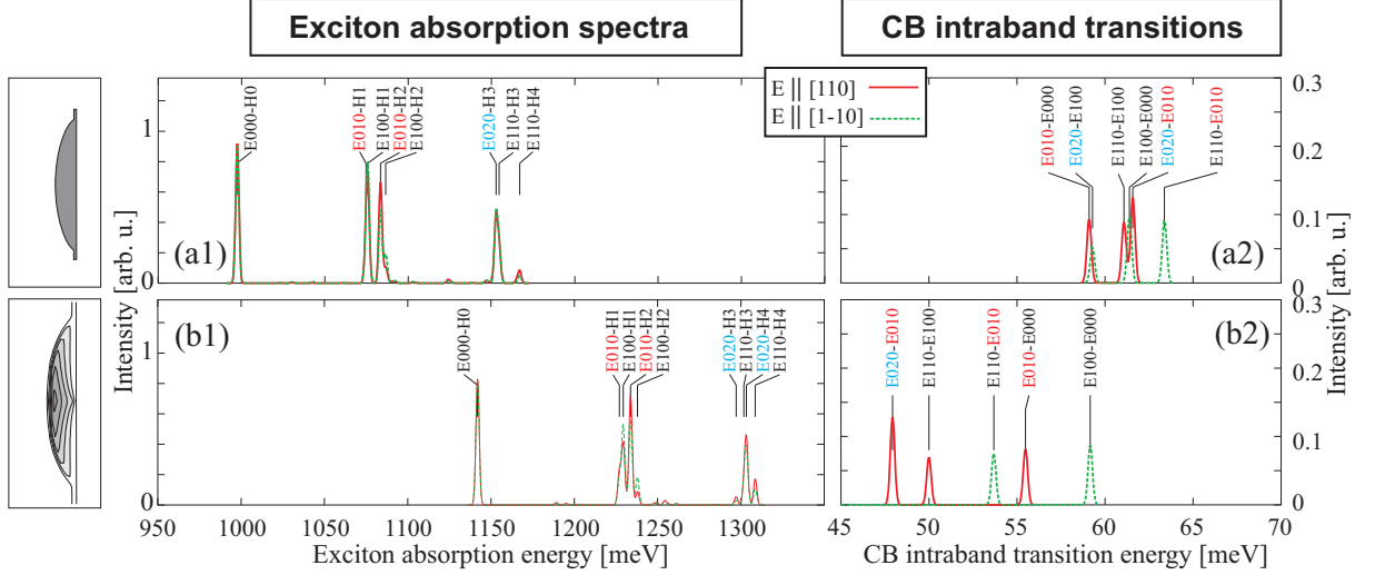
Figure 19: (Color online) Excitonic absorption spectra (left panel) and CB intraband transition spectra (right panel) shown for two QDs having a circular base. The first one is taken from series C and the other from series F , both having the same total amount of InAs inside the QD structure and a similar vertical aspect ratio of ar_V = 0.21 (a) and ar_V = 0.2 (b) respectively. First and second order piezoelectric effects are taken into account.
