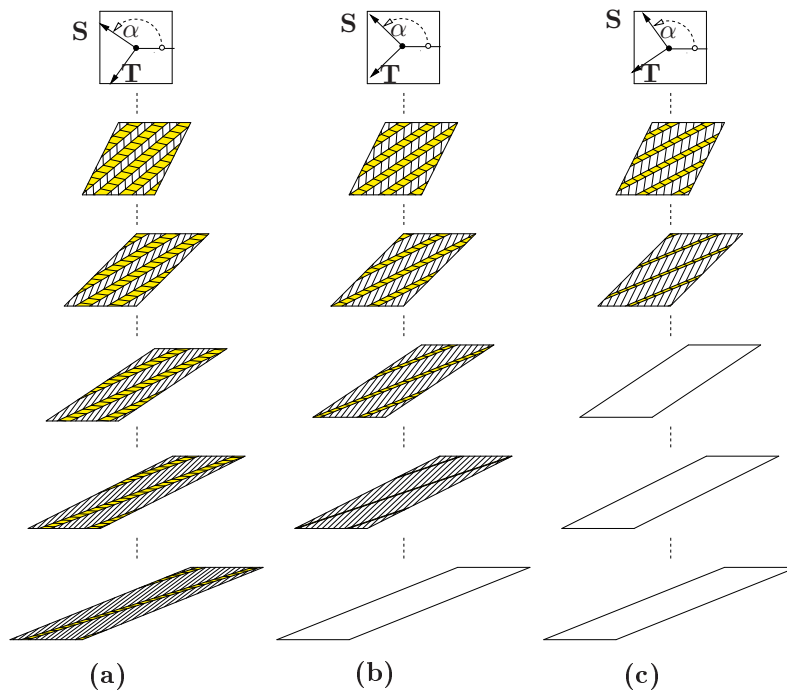
Figure 9: Simple shear test. Comparison of evolution of microstructures for simple shear test with three different slip system (a) \alpha = 145^\circ , (b) \alpha = 135^\circ , (c) \alpha = 125^\circ . After loss of material stability microstructures develop which are modeled as first-order rank-one laminates
