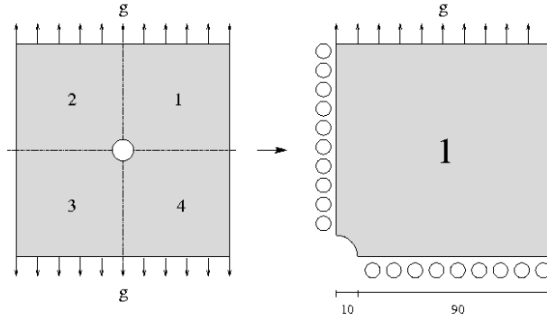
Figure 4: Here, the geometry of the example domain is outlined. Due to reasons of symmetry, only one of the quarters is solved.
