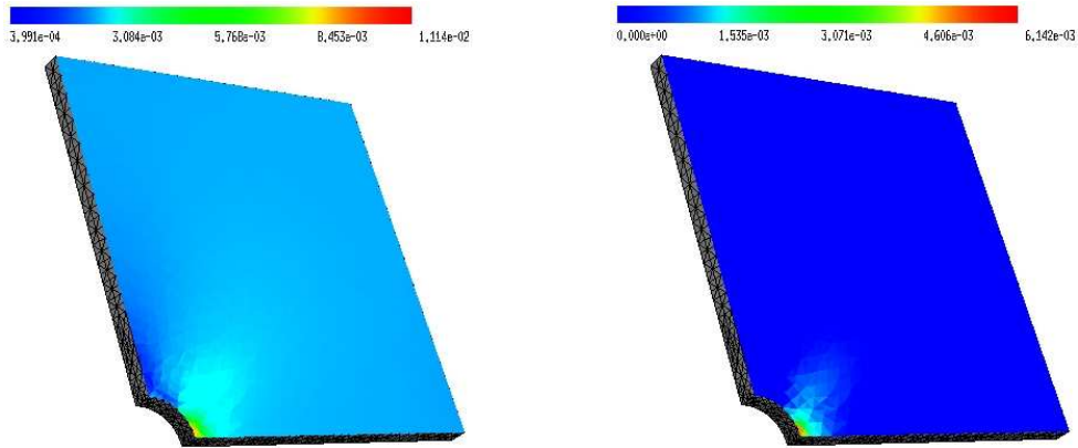
Figure 5: The Frobenius norms of the total strain \varepsilon (left) and of the plastic strain p (right).
