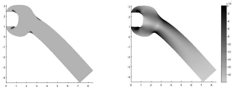
Figure 3: Elastoplastic zones (left) and yield function (right) of the deformed wrench geometry. The displacement is magnified by a factor 10 for visualization reasons.
