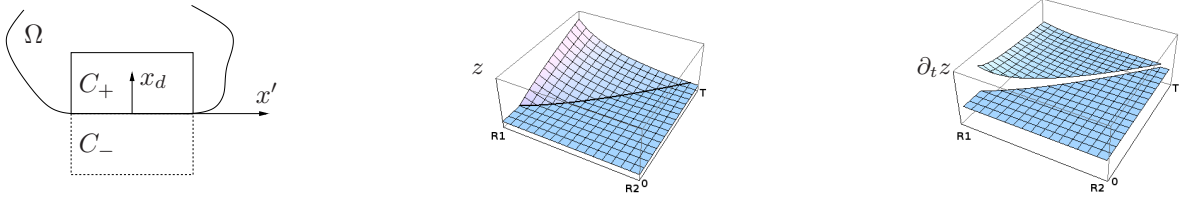
Figure 1: Example for the notation in Section 3.1.3 (left); Graph of the solution z : (0, T) \times (R_1, R_2) \rightarrow \mathbb{R} (middle) and of the time derivative \partial_t z (right).
