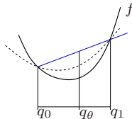
Figure 6: Uniformly convex function.
