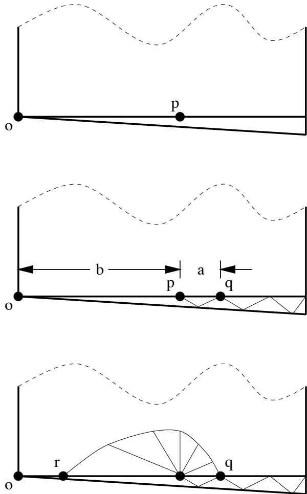
Figure 16: Top: A difficult PSLG with a small interior angle \phi . Center: The point p and the angle constraint necessitate the insertion of the point q . Bottom: The point q and the angle constraint necessitate the insertion of the point r . The process repeats eternally.
