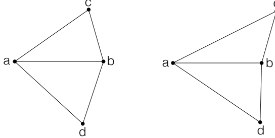
FIGURE 5. Left: edge ab is flippable. Right: edge ab is unflippable.
