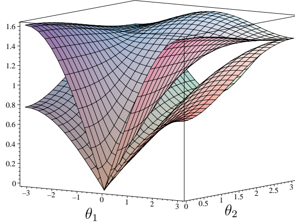
Figure 6.6: The two dispersion relations for the two-dimensional lattice (one half of \mathcal{T}_{\Gamma^*} is displayed only).
