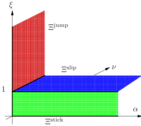
FIGURE 1. The set \Xi = \Xi^{\text{stick}} \cup \Xi^{\text{slip}} \cup \Xi^{\text{jump}}
