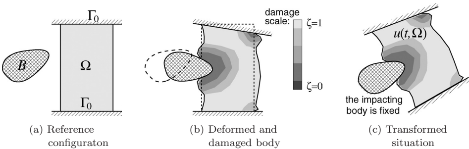
Fig. 1. A schematic situation of a moving rigid obstacle B impacting an elastic body undergoing possibly a damage due to this impact and the hard-device load on the part \Gamma_0 of the boundary \partial\Omega .
