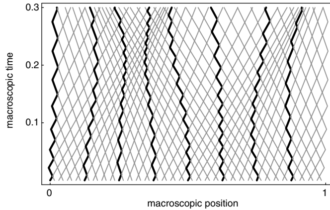
Figure 3. The microscopic dynamics in the macroscopic Euler representation for N = 64 . The trajectories of eight selected particles are drawn in black.
