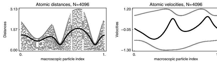
Figure 4. The microscopic dynamics in the macroscopic Lagrange representation for N = 4096 . The atomic distances and velocities are depicted in grey against y , for fixed \tau = 0.3 . The black lines represent the macroscopic mean values, whose dynamics is governed by the modulation system.
