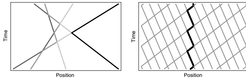
Figure 2. Left. Schematic representation of the microscopic dynamics in the Euler representation. Any particle moves along a zig-zag curve on the free flight trajectories of phonons. Right. Schematic representation of a travelling in the microscopic Euler representation with periodic boundary conditions.
