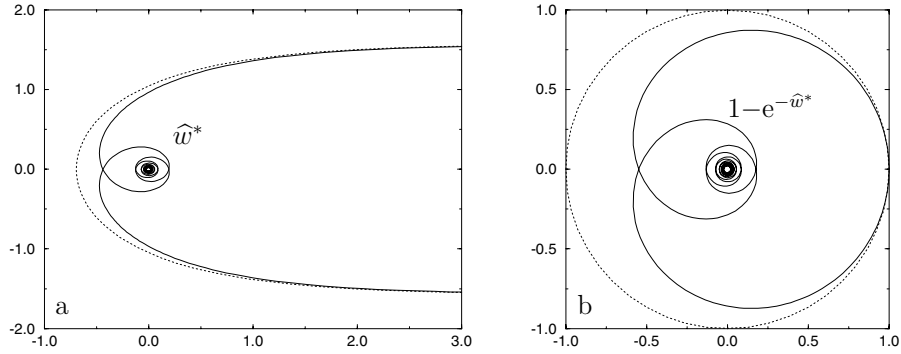
Fig. 2. (a) The region D \subset \mathbb{C} delimited by the dotted line contains the curve \{\hat{w}^*(\xi) \mid \xi \in \mathbb{R}\} (solid line). (b) The curve \{1 - e^{-\hat{w}^*(\xi)} \mid \xi \in \mathbb{R}\} (solid line) is contained in the unit disk of \mathbb{C} .
