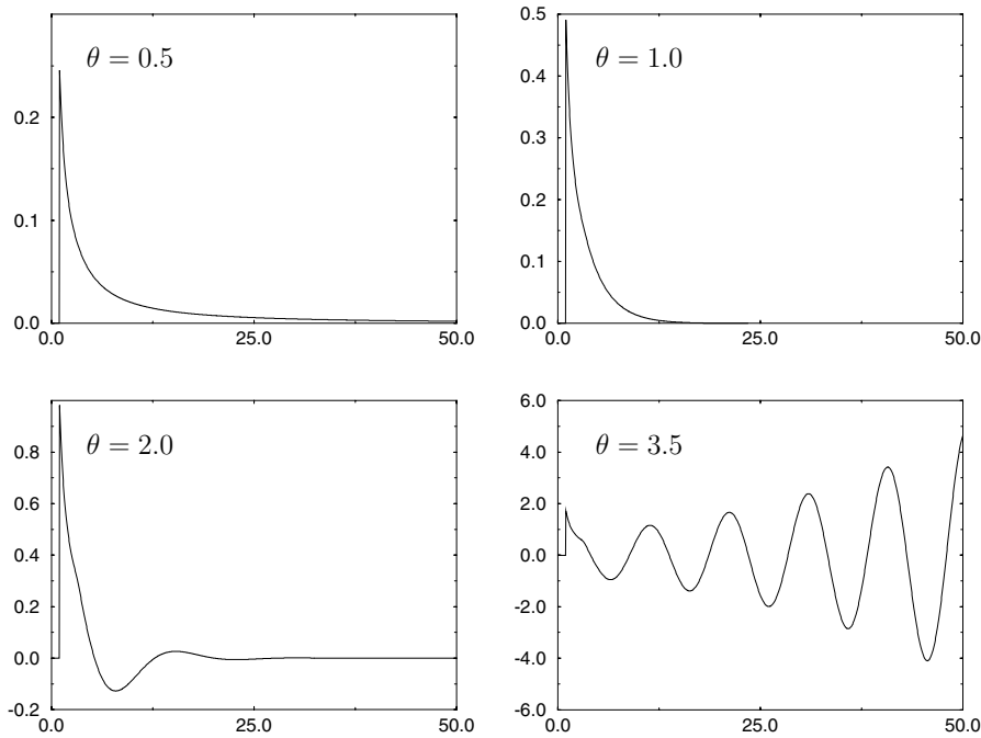
Fig. 1. The steady state \eta_\theta^* of the coarsening equation (3.3) with Q(z) = z^2 is represented for four values of the parameter \theta . The first two graphs ( \theta = 0.5 and \theta = 1.0 ) illustrate the conclusions of Theorem 4.6, and the other two ( \theta = 2.0 and \theta = 3.5 ) illustrate the remarks after Lemma 4.7. The pictures were produced using the explicit formula (1.6) and a FFT routine to compute the Fourier transforms.
