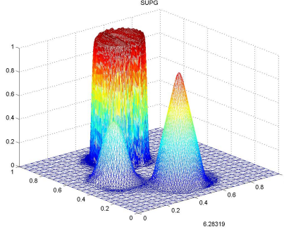
Fig. 9. Example 4. Approximation at time 2\pi obtained with the error estimator (10) and the corresponding mesh.
