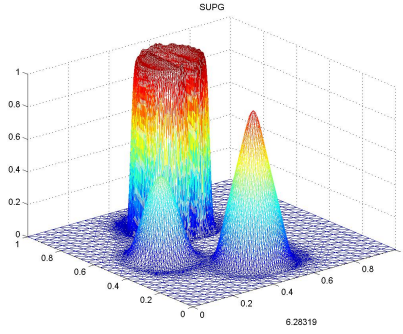
Fig. 10. Example 4. Approximation at time 2\pi obtained with the error estimator (11) and the corresponding mesh.
