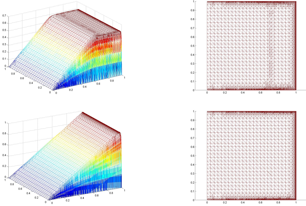
Fig. 3. Example 3. Solution computed with the SUPG-based method (left) and corresponding adaptive mesh (right), at time t = 0.6 (top) and t = 1.2 (bottom).
