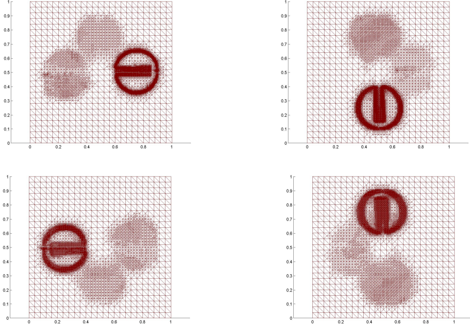
Fig. 8. Example 4. SUPG-based method, computational meshes at times t \in \{\pi/2, \pi, 3\pi/2, 2\pi\} .
