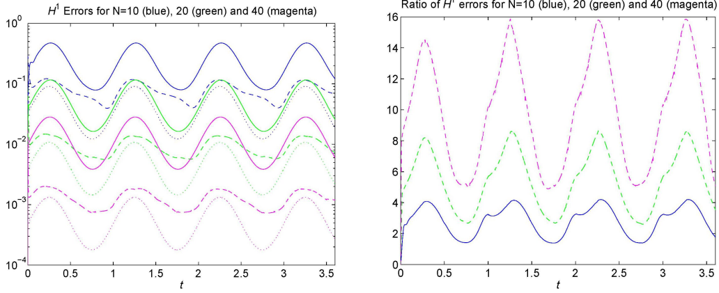
Fig. 1. Left: H^1(\Omega) norm of the convective derivative of the error for u_h (continuous line), \tilde{u}_h (discontinuous line), and w_h (dotted line). Right: ratios between the H^1(\Omega) norm of the convective derivative of the errors of u_h and \tilde{u}_h .
