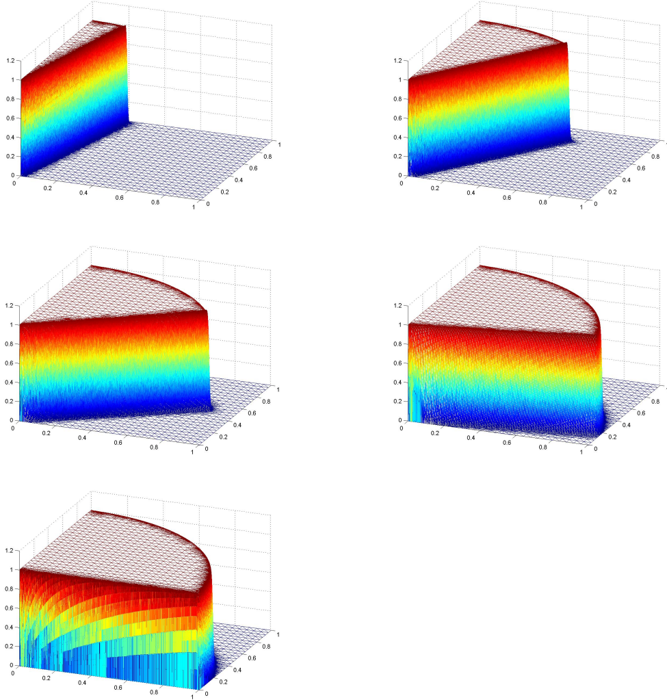
Fig. 12. Example 5. SUPG-based algorithm, solutions at times t \in \{0.2, 0.6, 1.0, 1.4, 1.8\} .
