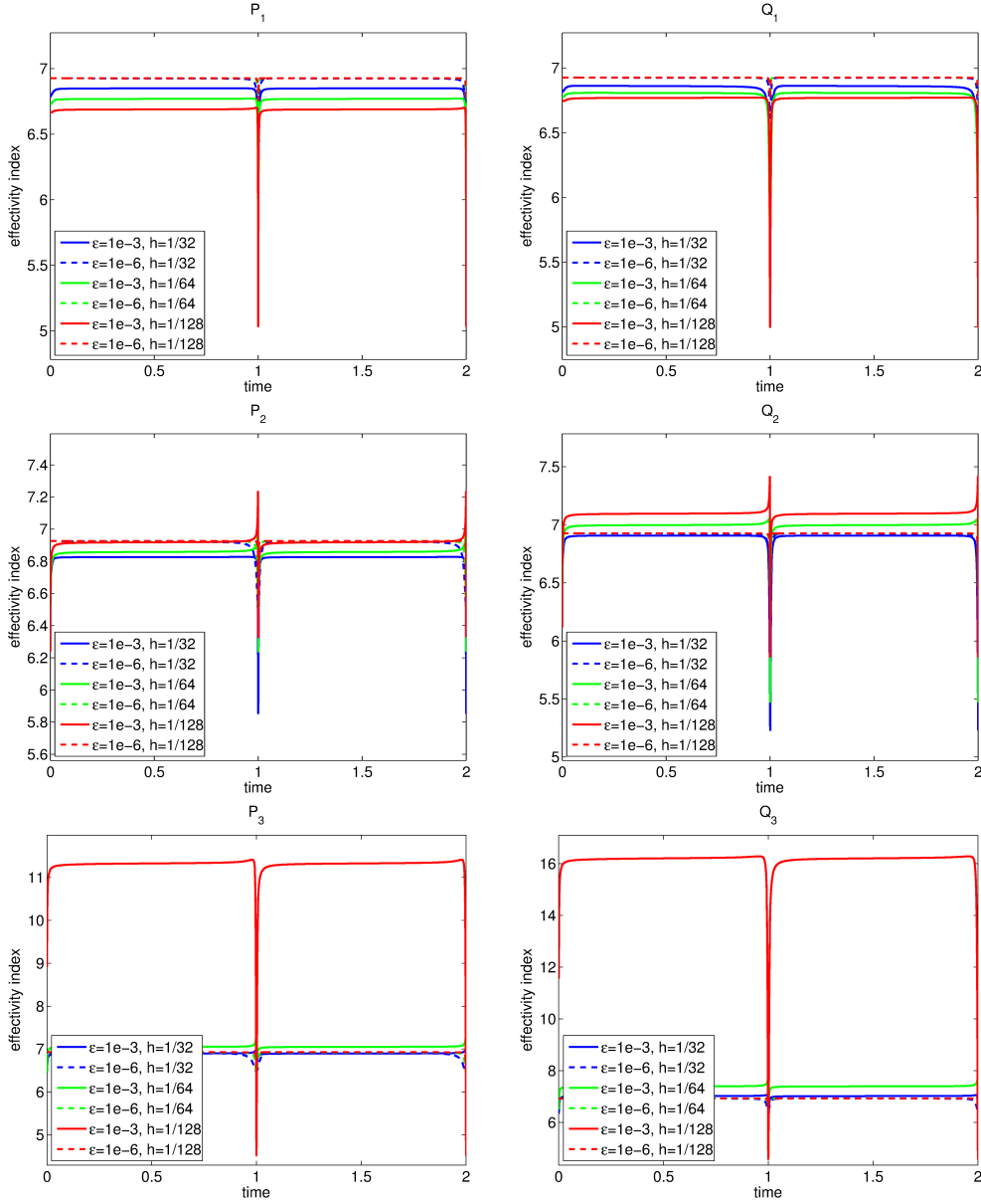
Fig. 2. Example 2. Effectivity indices.
