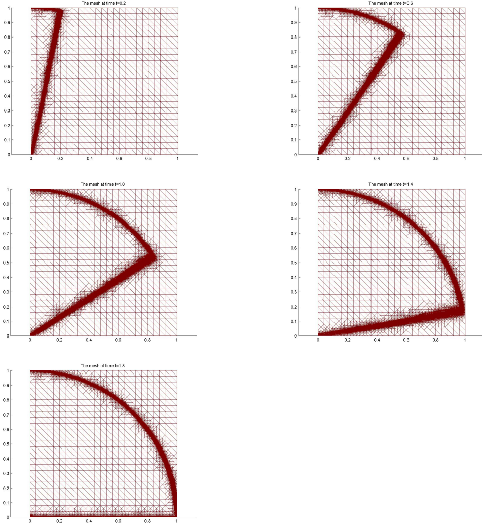
Fig. 13. Example 5. SUPG-based algorithm, meshes at times t \in \{0.2, 0.6, 1.0, 1.4, 1.8\} .
