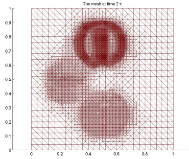
Fig. 10. Example 4. Approximation at time 2\pi obtained with the error estimator (11) and the corresponding mesh.
