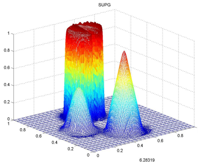
Fig. 11. Example 4. Approximation at time 2\pi obtained with the error estimator (12) and the corresponding mesh.
