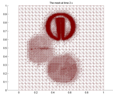
Fig. 11. Example 4. Approximation at time 2\pi obtained with the error estimator (12) and the corresponding mesh.
