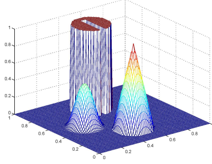
Fig. 6. Example 4. Initial condition
