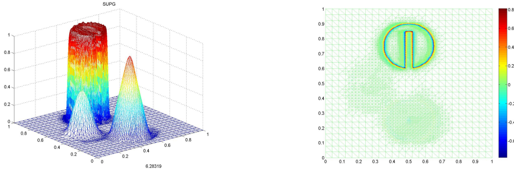
Fig. 7. Example 4. SUPG-based algorithm, approximation after one rotation (left) and difference to the initial condition (right).
