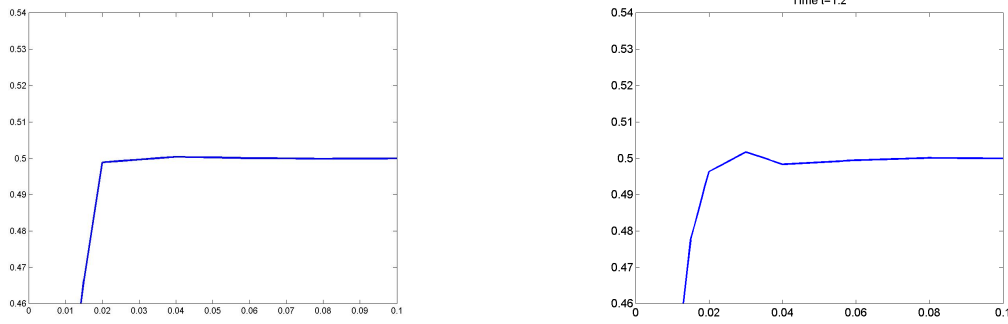
Fig. 5. Example 3. Zoom of the parabolic layer at x = 0.5 and y = 0 at time t = 1.2 , SUPG-based algorithm (left), Galerkin-based algorithm (right).
