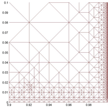
Fig. 4. Example 3. Zoom of bottom right picture of Figure 3.
