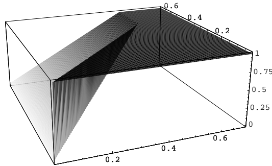
FIGURE 1. Cost function \xi \mapsto \Phi(\xi) from Example 1.
