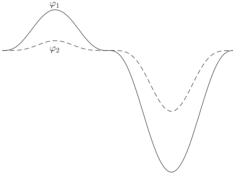
Fig. 1 Segments of graphs \varphi_1 and 2.3 \times 10^9 \varphi_2 . The constant in front of \varphi_2 is used for graphical purposes
