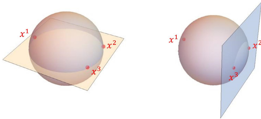
Fig. 1. Examples for spherical caps.
