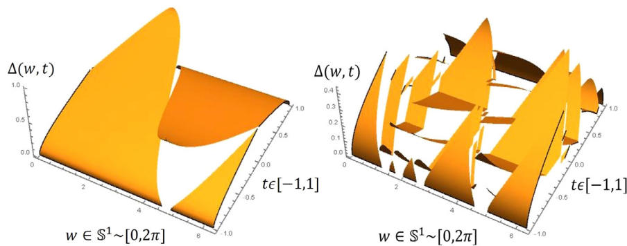
Fig. 2. Plot of \Delta(w, t) for a sample of size N = 1 (left) and N = 5 (right) on \mathbb{S}^1 .
