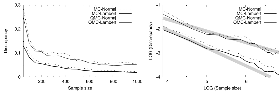
Fig. 4. Discrepancy as a function of sample size for 4 different sampling schemes in original form (left) and Log–Log Plot (right). For details see text.
