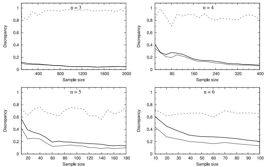
Fig. 3. Plot of discrepancy \Delta (thick line), of its lower estimate \tilde{\Delta} (thin line) and of the ratio \tilde{\Delta}/\Delta (dashed line) for different dimensions ( n = 3, 4, 5, 6 ) and sample sizes.
