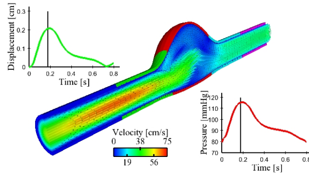
Figure 6: Snapshot of the velocity field inside the idealized AAA. The curves show outlet pressure and displacements of the aneurysm wall.
